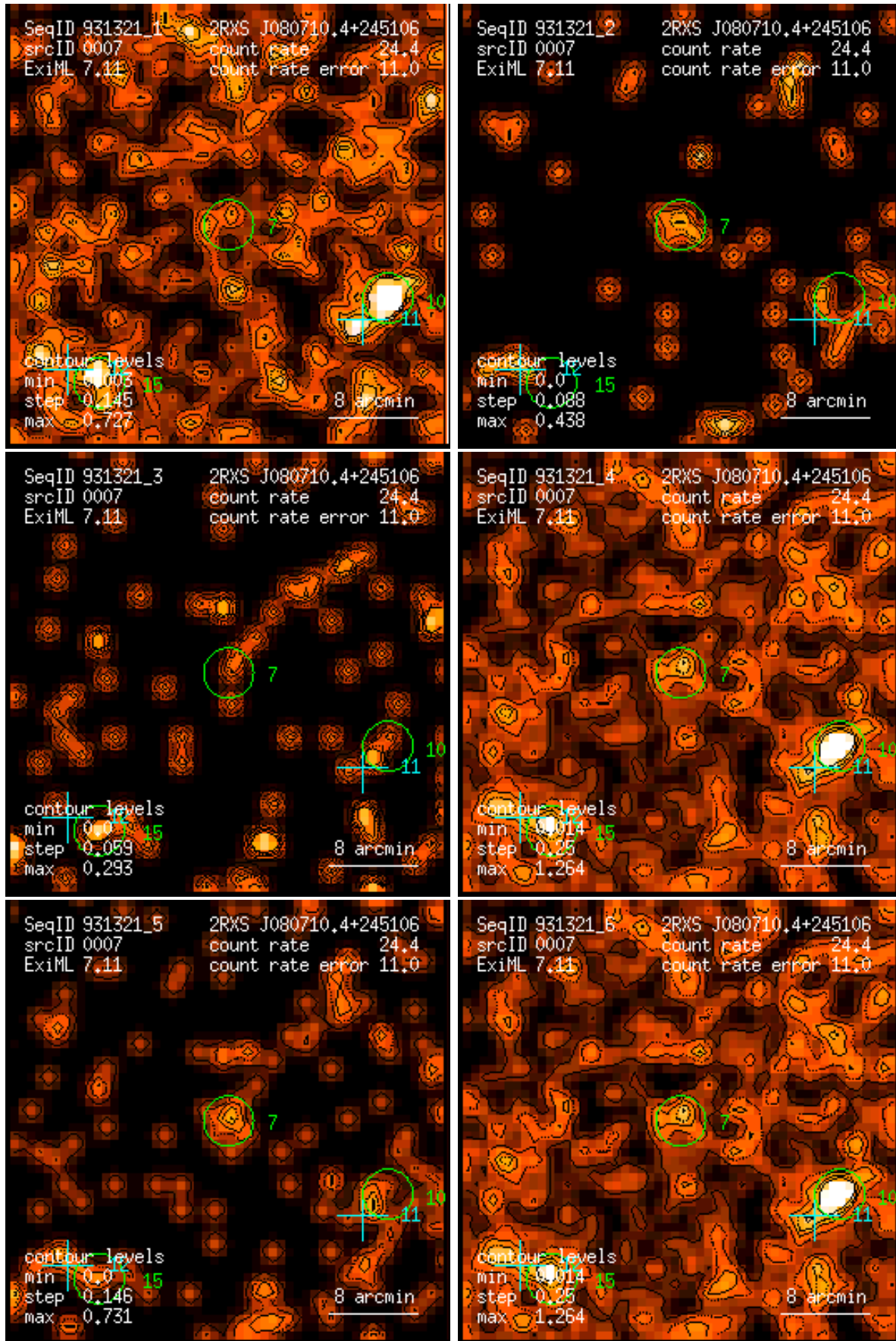
Figure 7: RASS 931321: detection 0007: band rate images, Gaussian filter: (1) PSPC channels 11 – 41, (2) 52 – 90, (3) 91 – 201, (4) 11 – 235, (5) 52 – 201, (6) 11 – 201. Broad band rates in counts/ks. Band rate contour levels in counts/ks/arcmin 2 .
