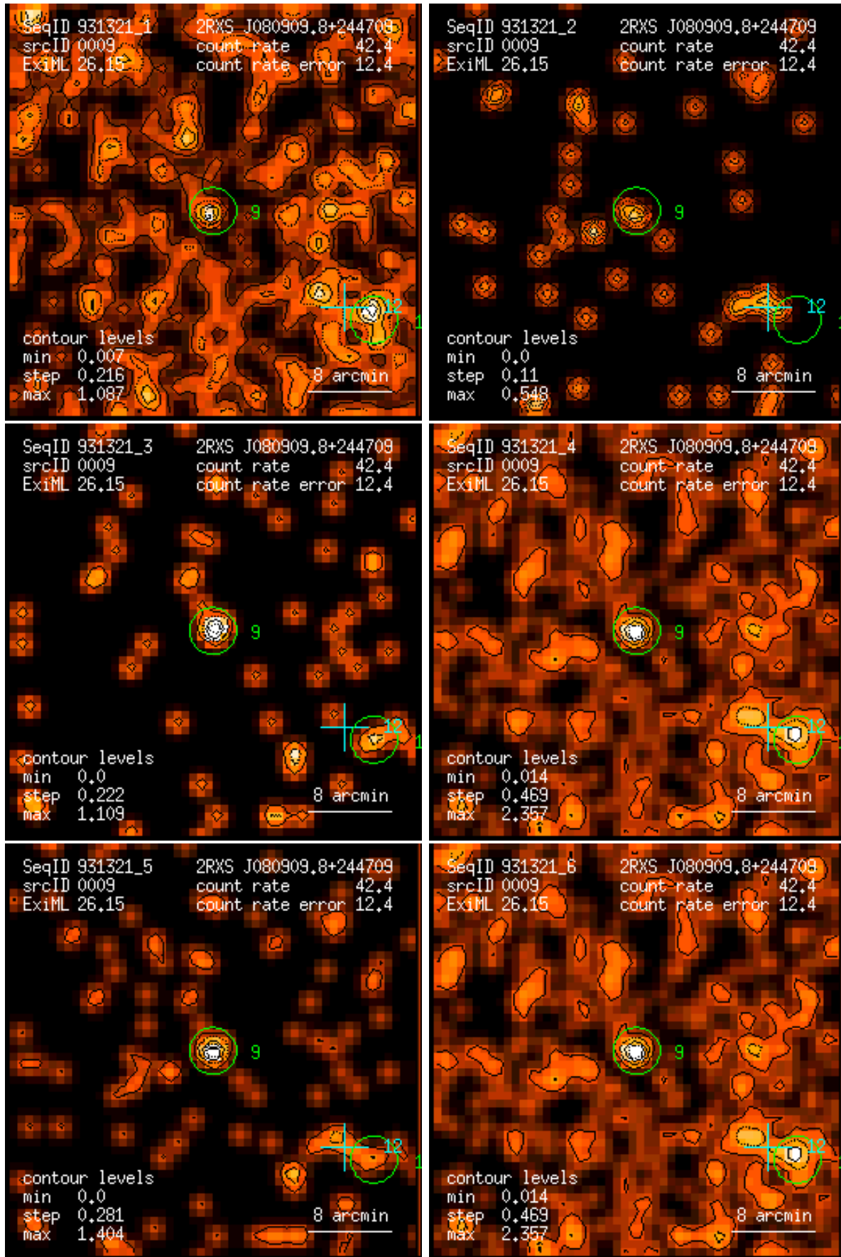
Figure 9: RASS 931321: detection 0009: band rate images, Gaussian filter: (1) PSPC channels 11 – 41, (2) 52 – 90, (3) 91 – 201, (4) 11 – 235, (5) 52 – 201, (6) 11 – 201. Broad band rates in counts/ks. Band rate contour levels in counts/ks/arcmin 2 .
