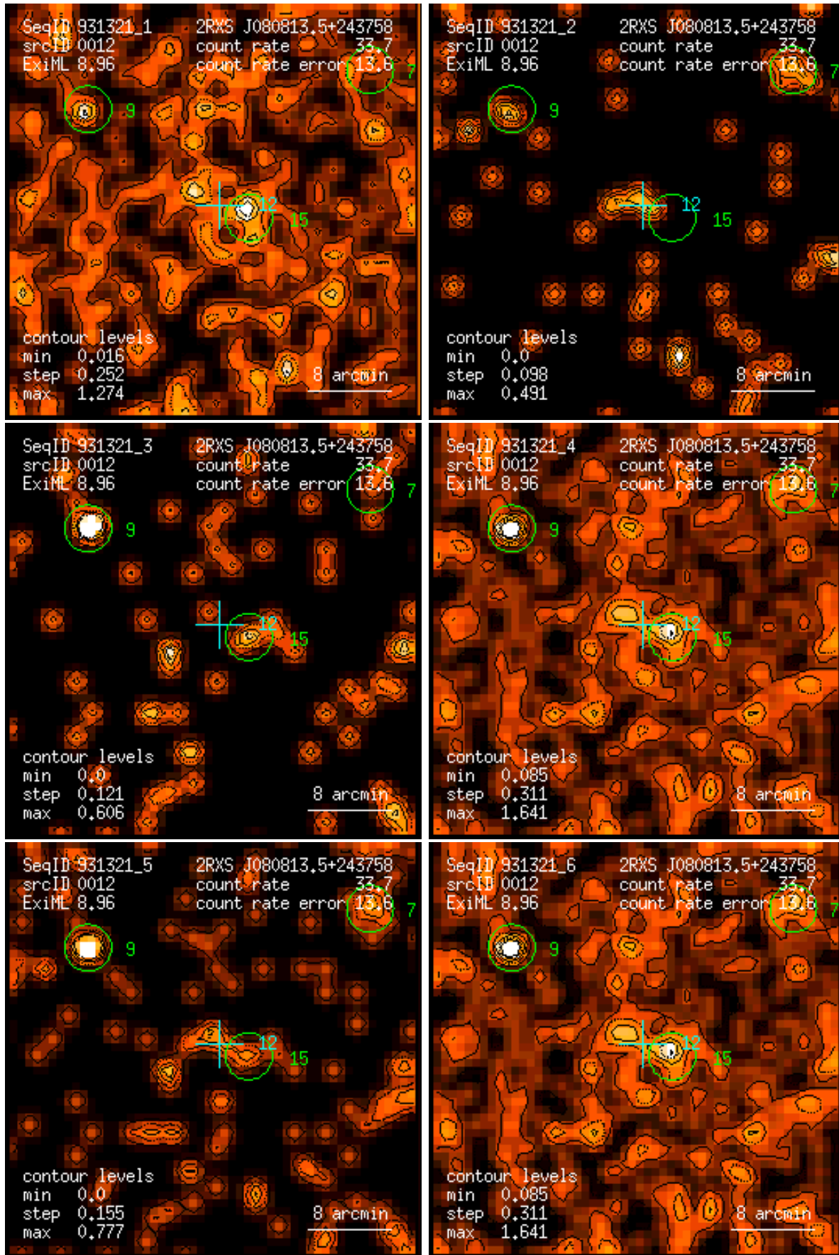
Figure 12: RASS 931321: detection 0012: band rate images, Gaussian filter: (1) PSPC channels 11 – 41, (2) 52 – 90, (3) 91 – 201, (4) 11 – 235, (5) 52 – 201, (6) 11 – 201. Broad band rates in counts/ks. Band rate contour levels in counts/ks/arcmin 2 .
