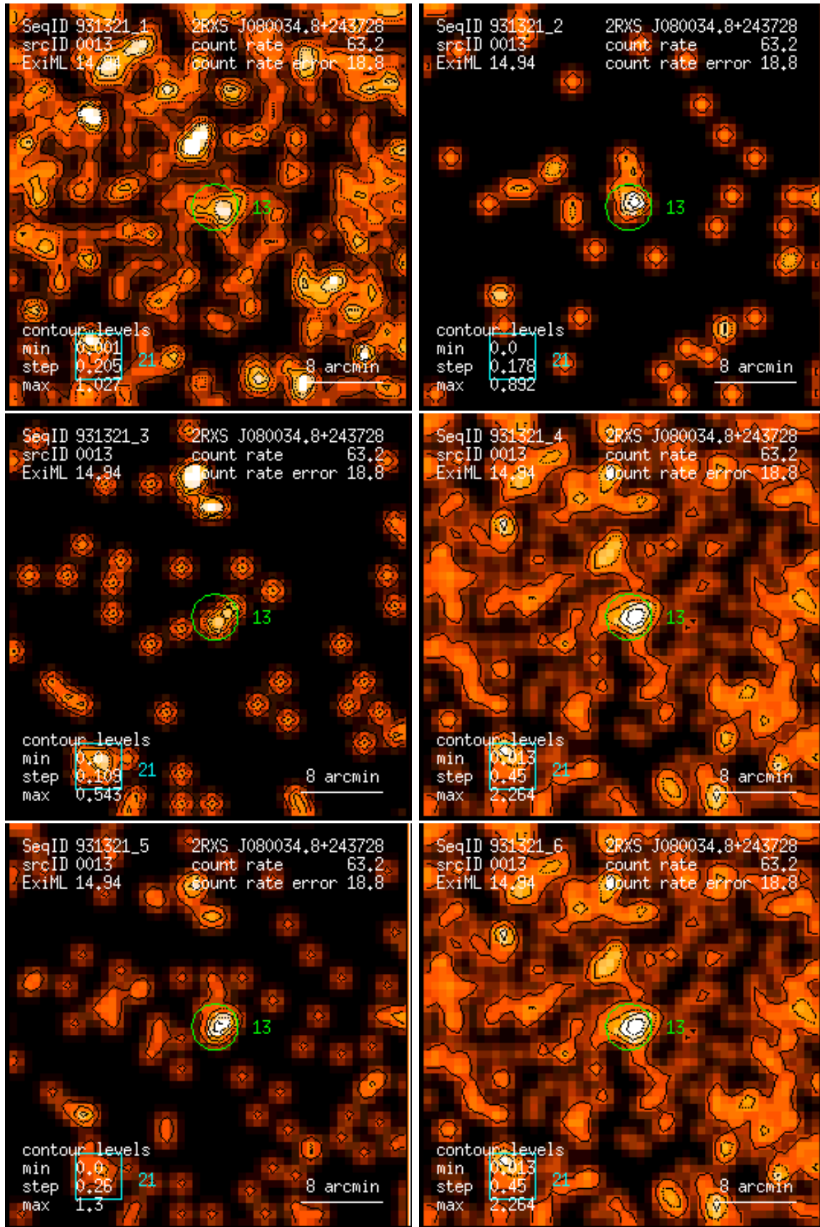
Figure 13: RASS 931321: detection 0013: band rate images, Gaussian filter: (1) PSPC channels 11 – 41, (2) 52 – 90, (3) 91 – 201, (4) 11 – 235, (5) 52 – 201, (6) 11 – 201. Broad band rates in counts/ks. Band rate contour levels in counts/ks/arcmin 2 .
