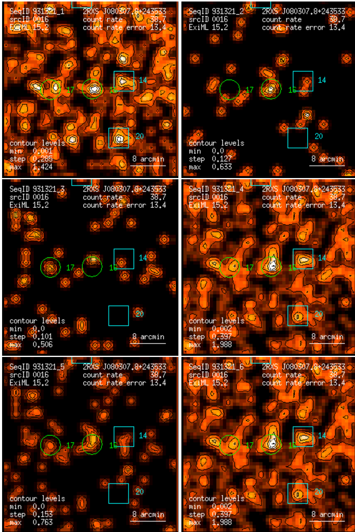
Figure 16: RASS 931321: detection 0016: band rate images, Gaussian filter: (1) PSPC channels 11 – 41, (2) 52 – 90, (3) 91 – 201, (4) 11 – 235, (5) 52 – 201, (6) 11 – 201. Broad band rates in counts/ks. Band rate contour levels in counts/ks/arcmin 2 .
