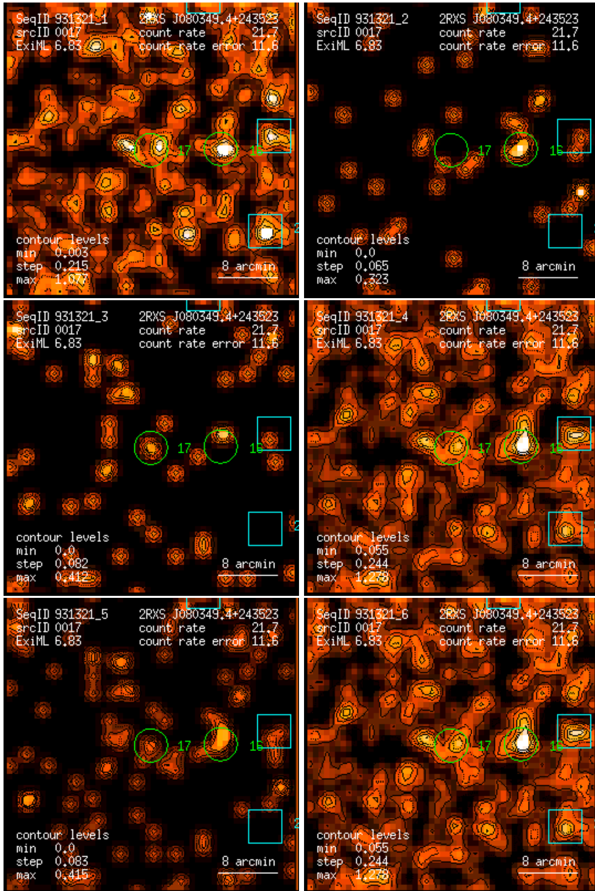
Figure 17: RASS 931321: detection 0017: band rate images, Gaussian filter: (1) PSPC channels 11 – 41, (2) 52 – 90, (3) 91 – 201, (4) 11 – 235, (5) 52 – 201, (6) 11 – 201. Broad band rates in counts/ks. Band rate contour levels in counts/ks/arcmin 2 .
