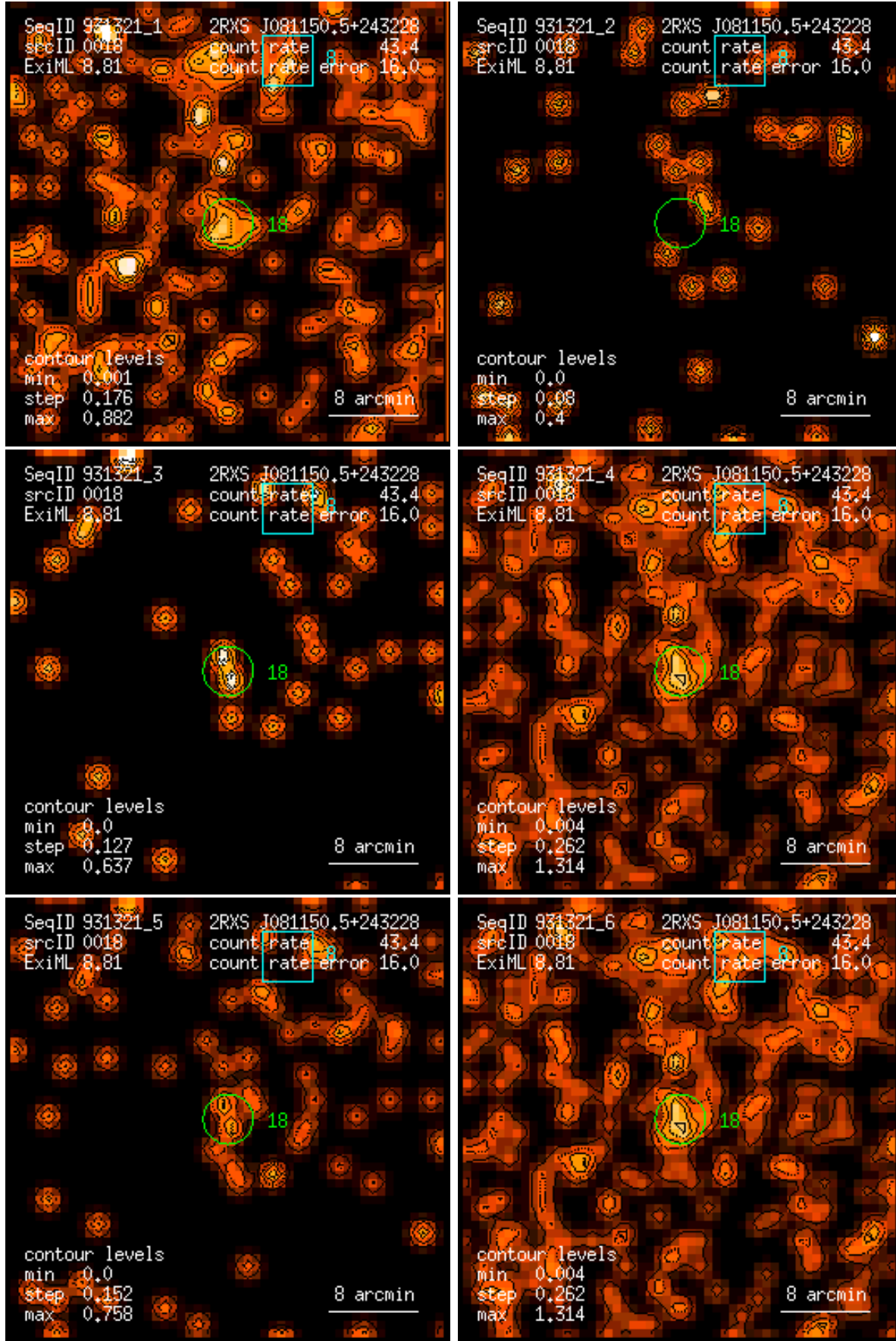
Figure 18: RASS 931321: detection 0018: band rate images, Gaussian filter: (1) PSPC channels 11 – 41, (2) 52 – 90, (3) 91 – 201, (4) 11 – 235, (5) 52 – 201, (6) 11 – 201. Broad band rates in counts/ks. Band rate contour levels in counts/ks/arcmin 2 .
