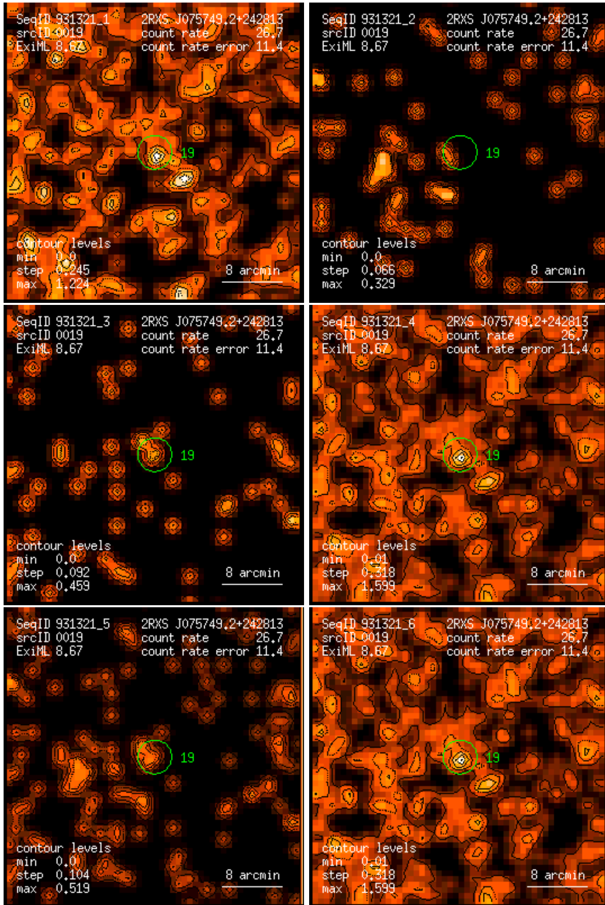
Figure 19: RASS 931321: detection 0019: band rate images, Gaussian filter: (1) PSPC channels 11 – 41, (2) 52 – 90, (3) 91 – 201, (4) 11 – 235, (5) 52 – 201, (6) 11 – 201. Broad band rates in counts/ks. Band rate contour levels in counts/ks/arcmin 2 .
