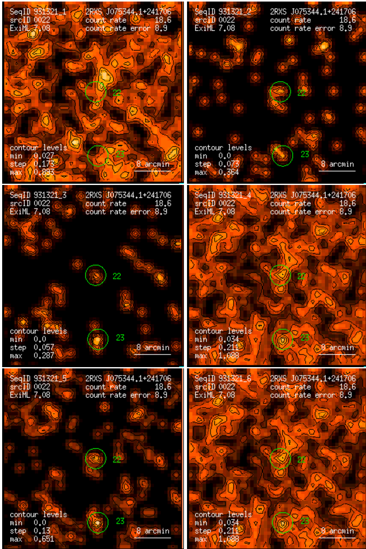
Figure 22: RASS 931321: detection 0022: band rate images, Gaussian filter: (1) PSPC channels 11 – 41, (2) 52 – 90, (3) 91 – 201, (4) 11 – 235, (5) 52 – 201, (6) 11 – 201. Broad band rates in counts/ks. Band rate contour levels in counts/ks/arcmin 2 .
