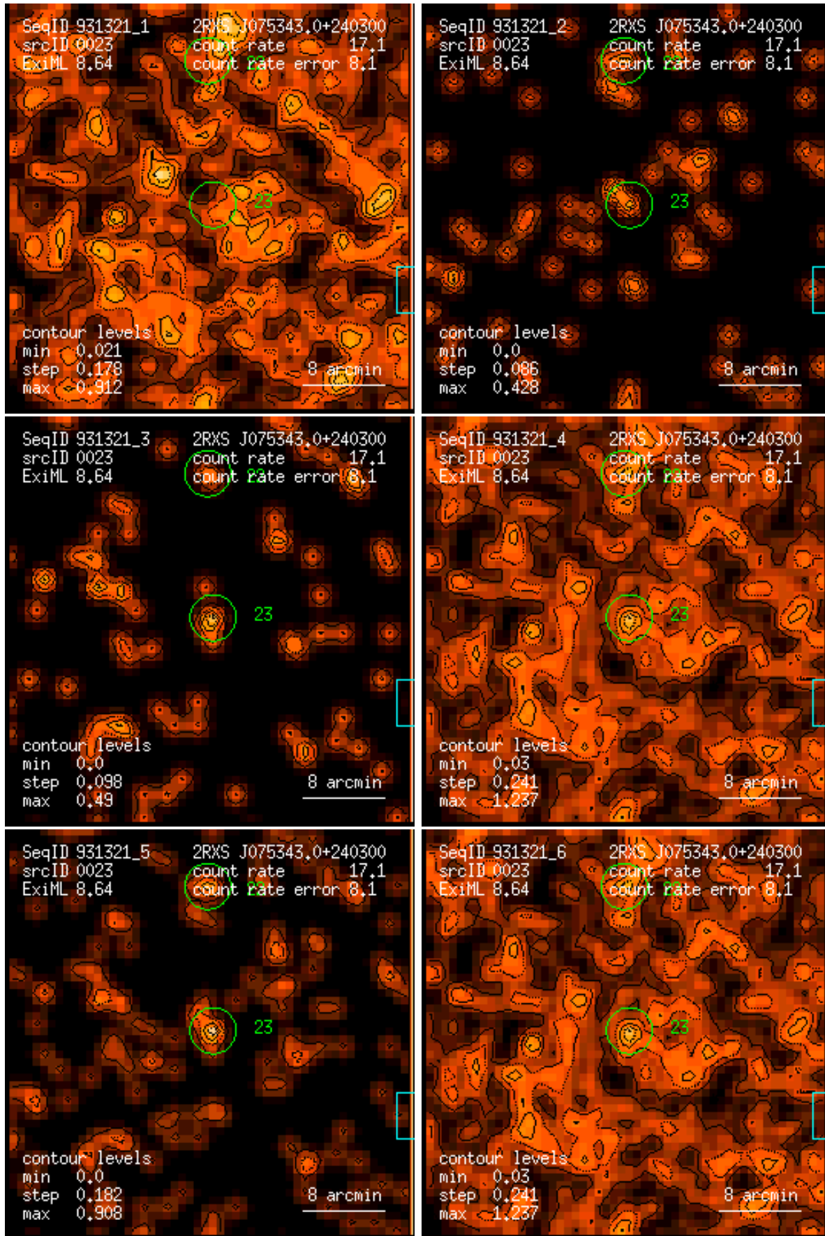
Figure 23: RASS 931321: detection 0023: band rate images, Gaussian filter: (1) PSPC channels 11 – 41, (2) 52 – 90, (3) 91 – 201, (4) 11 – 235, (5) 52 – 201, (6) 11 – 201. Broad band rates in counts/ks. Band rate contour levels in counts/ks/arcmin 2 .
