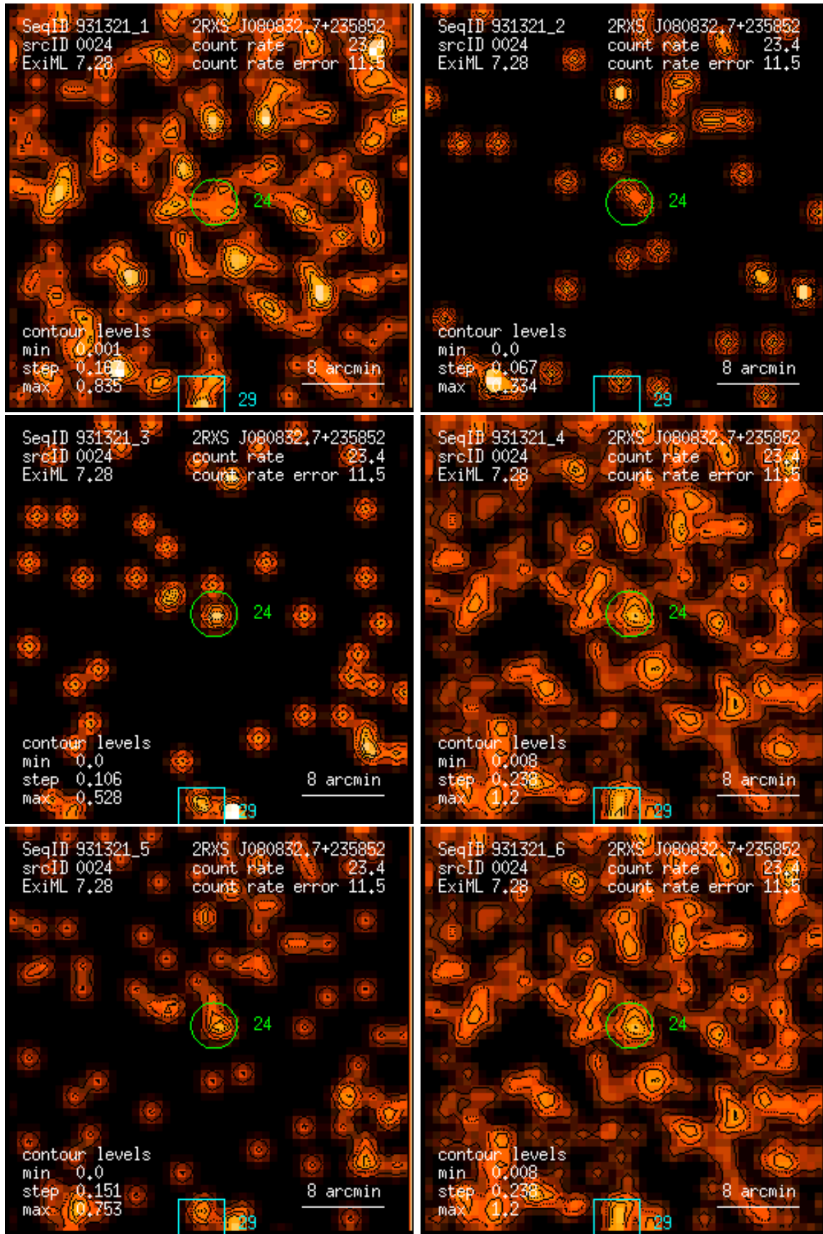
Figure 24: RASS 931321: detection 0024: band rate images, Gaussian filter: (1) PSPC channels 11 – 41, (2) 52 – 90, (3) 91 – 201, (4) 11 – 235, (5) 52 – 201, (6) 11 – 201. Broad band rates in counts/ks. Band rate contour levels in counts/ks/arcmin 2 .
