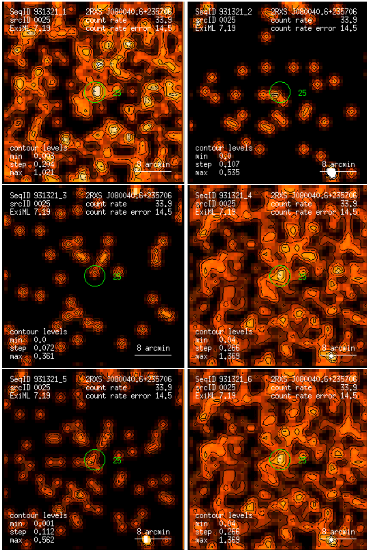
Figure 25: RASS 931321: detection 0025: band rate images, Gaussian filter: (1) PSPC channels 11 – 41, (2) 52 – 90, (3) 91 – 201, (4) 11 – 235, (5) 52 – 201, (6) 11 – 201. Broad band rates in counts/ks. Band rate contour levels in counts/ks/arcmin 2 .
