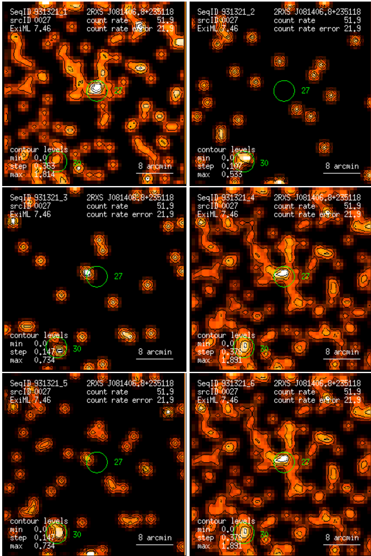
Figure 27: RASS 931321: detection 0027: band rate images, Gaussian filter: (1) PSPC channels 11 – 41, (2) 52 – 90, (3) 91 – 201, (4) 11 – 235, (5) 52 – 201, (6) 11 – 201. Broad band rates in counts/ks. Band rate contour levels in counts/ks/arcmin 2 .
