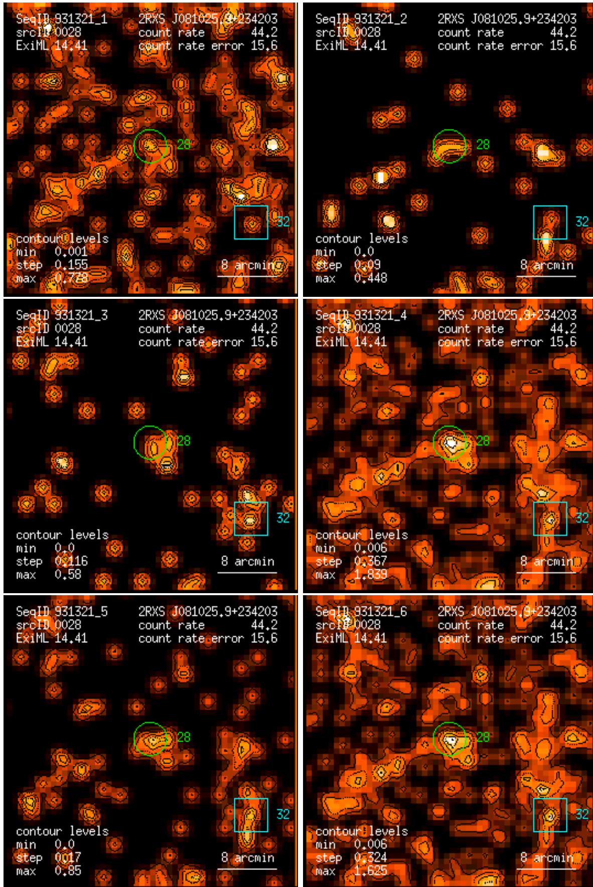
Figure 28: RASS 931321: detection 0028: band rate images, Gaussian filter: (1) PSPC channels 11 – 41, (2) 52 – 90, (3) 91 – 201, (4) 11 – 235, (5) 52 – 201, (6) 11 – 201. Broad band rates in counts/ks. Band rate contour levels in counts/ks/arcmin 2 .
