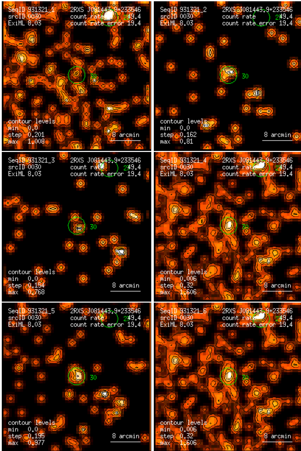
Figure 30: RASS 931321: detection 0030: band rate images, Gaussian filter: (1) PSPC channels 11 – 41, (2) 52 – 90, (3) 91 – 201, (4) 11 – 235, (5) 52 – 201, (6) 11 – 201. Broad band rates in counts/ks. Band rate contour levels in counts/ks/arcmin 2 .
