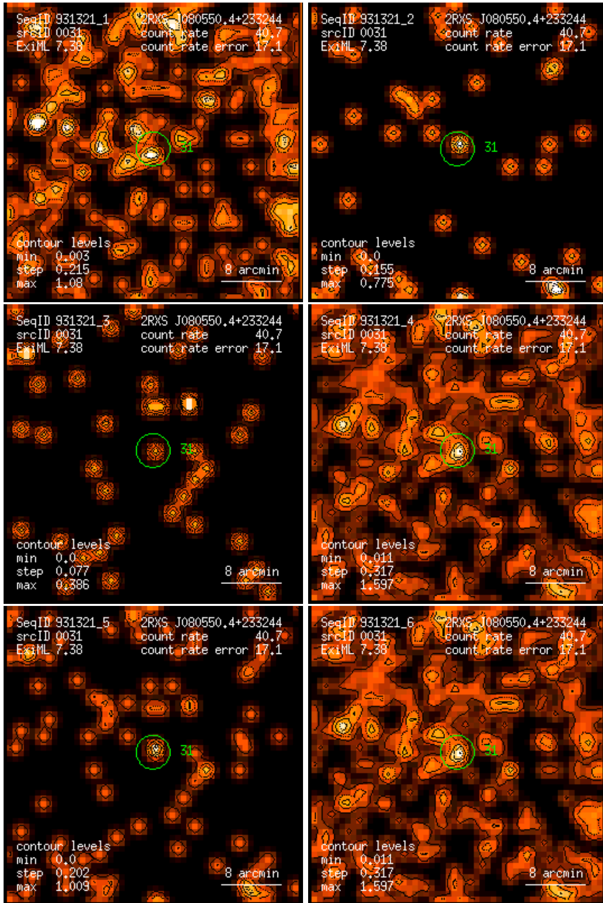
Figure 31: RASS 931321: detection 0031: band rate images, Gaussian filter: (1) PSPC channels 11 – 41, (2) 52 – 90, (3) 91 – 201, (4) 11 – 235, (5) 52 – 201, (6) 11 – 201. Broad band rates in counts/ks. Band rate contour levels in counts/ks/arcmin 2 .
