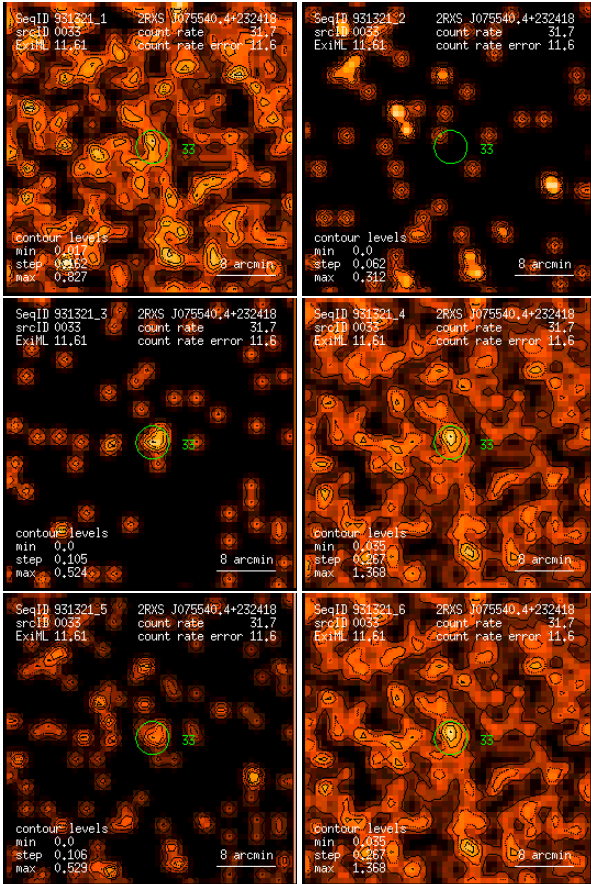
Figure 33: RASS 931321: detection 0033: band rate images, Gaussian filter: (1) PSPC channels 11 – 41, (2) 52 – 90, (3) 91 – 201, (4) 11 – 235, (5) 52 – 201, (6) 11 – 201. Broad band rates in counts/ks. Band rate contour levels in counts/ks/arcmin 2 .
