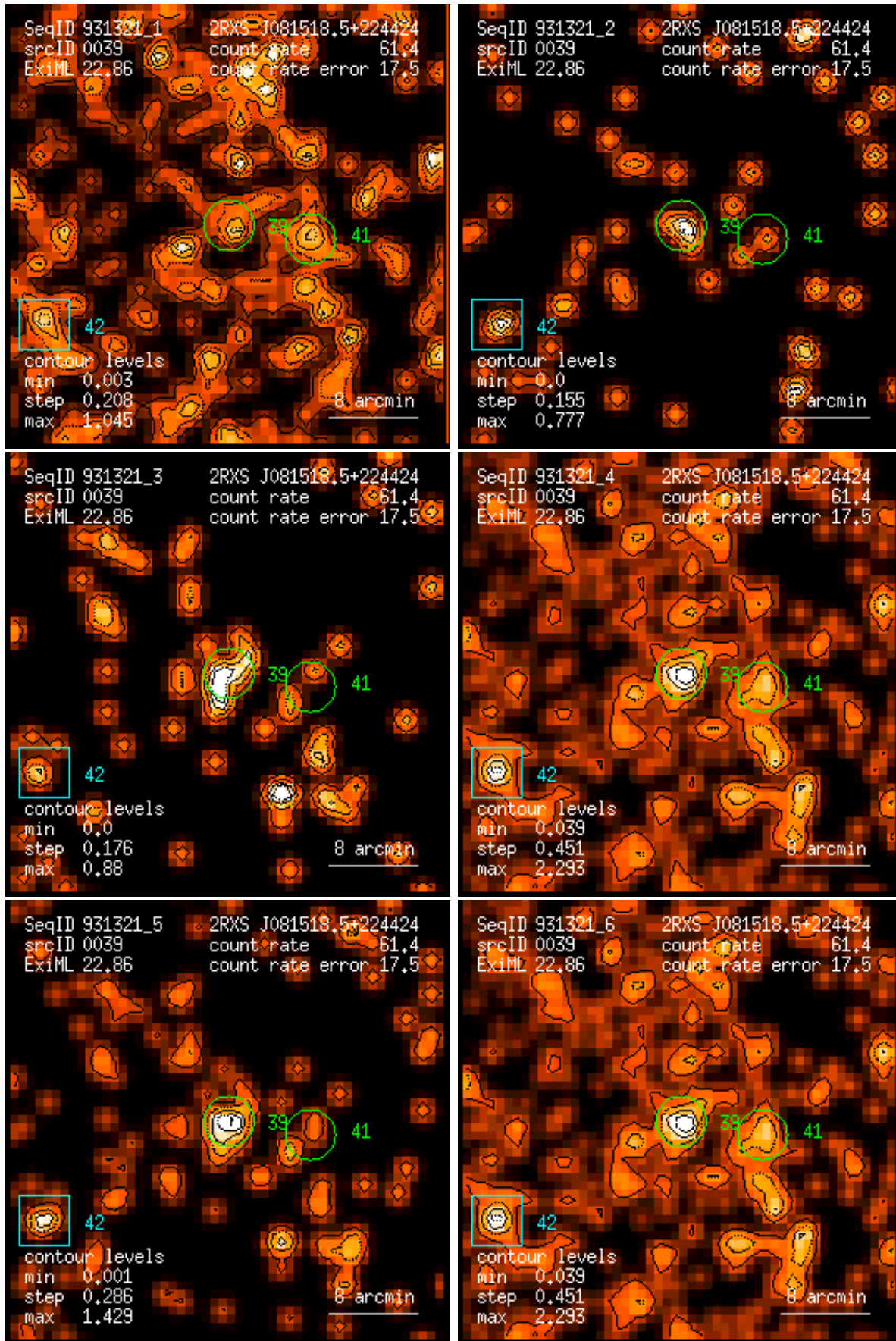
Figure 39: RASS 931321: detection 0039: band rate images, Gaussian filter: (1) PSPC channels 11 – 41, (2) 52 – 90, (3) 91 – 201, (4) 11 – 235, (5) 52 – 201, (6) 11 – 201. Broad band rates in counts/ks. Band rate contour levels in counts/ks/arcmin 2 .
