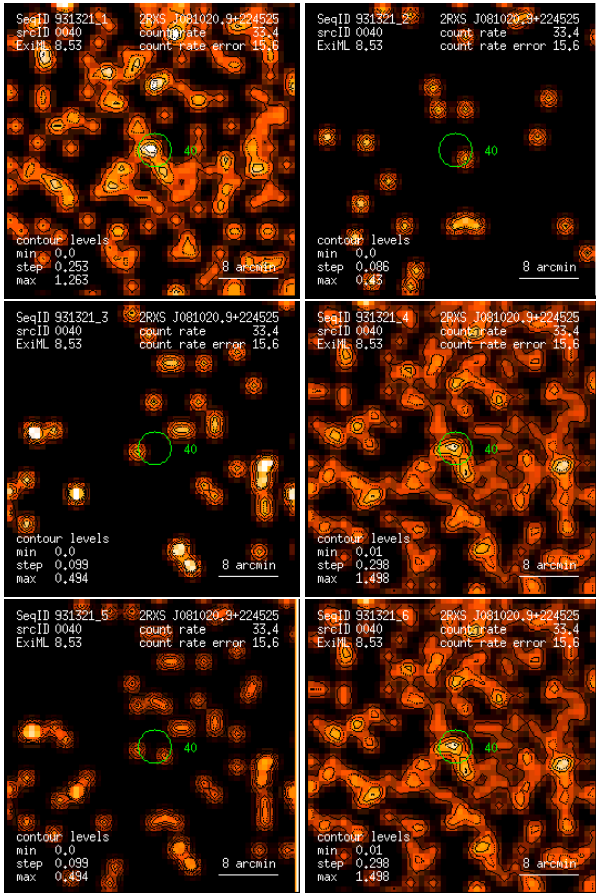
Figure 40: RASS 931321: detection 0040: band rate images, Gaussian filter: (1) PSPC channels 11 – 41, (2) 52 – 90, (3) 91 – 201, (4) 11 – 235, (5) 52 – 201, (6) 11 – 201. Broad band rates in counts/ks. Band rate contour levels in counts/ks/arcmin 2 .
