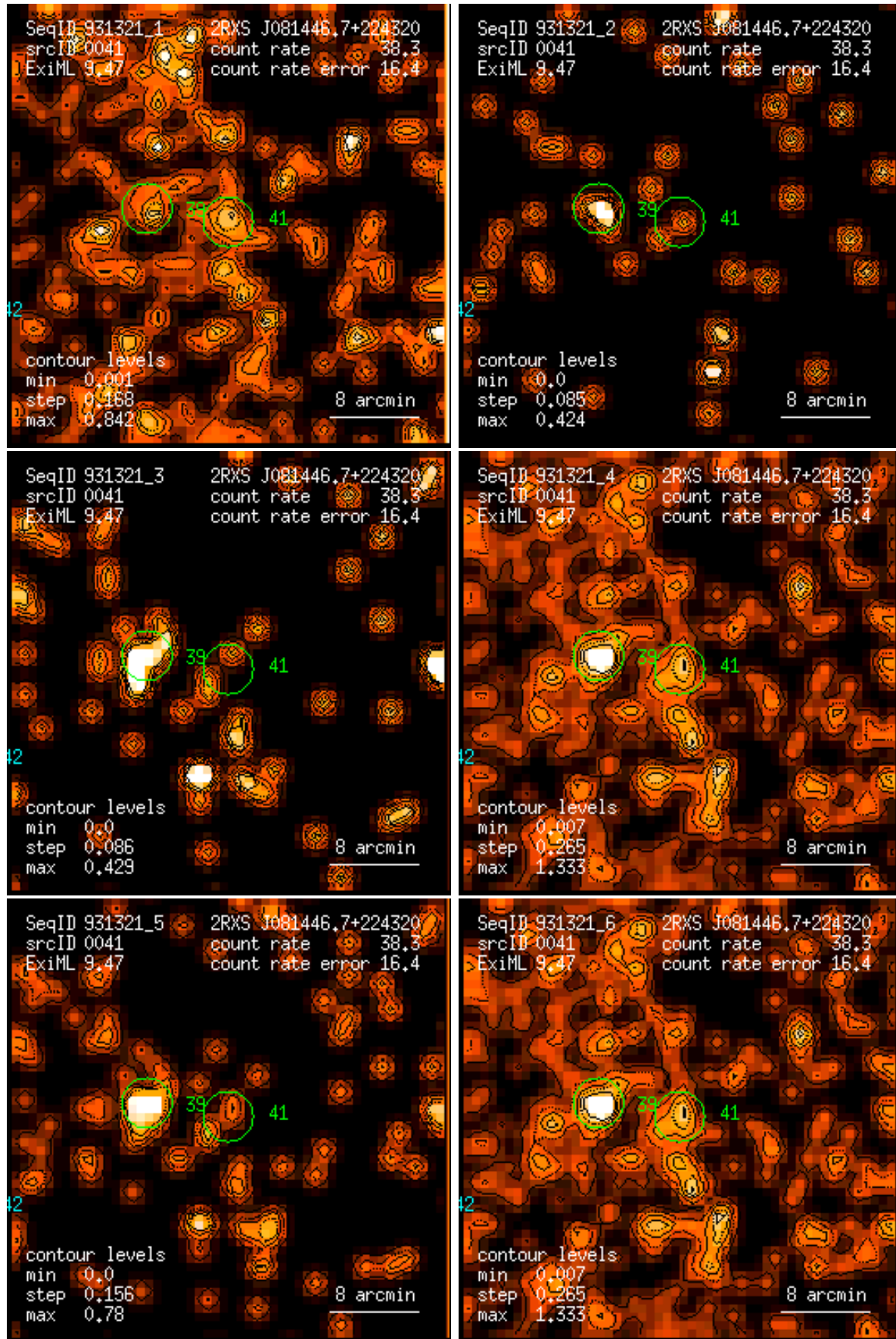
Figure 41: RASS 931321: detection 0041: band rate images, Gaussian filter: (1) PSPC channels 11 – 41, (2) 52 – 90, (3) 91 – 201, (4) 11 – 235, (5) 52 – 201, (6) 11 – 201. Broad band rates in counts/ks. Band rate contour levels in counts/ks/arcmin 2 .
