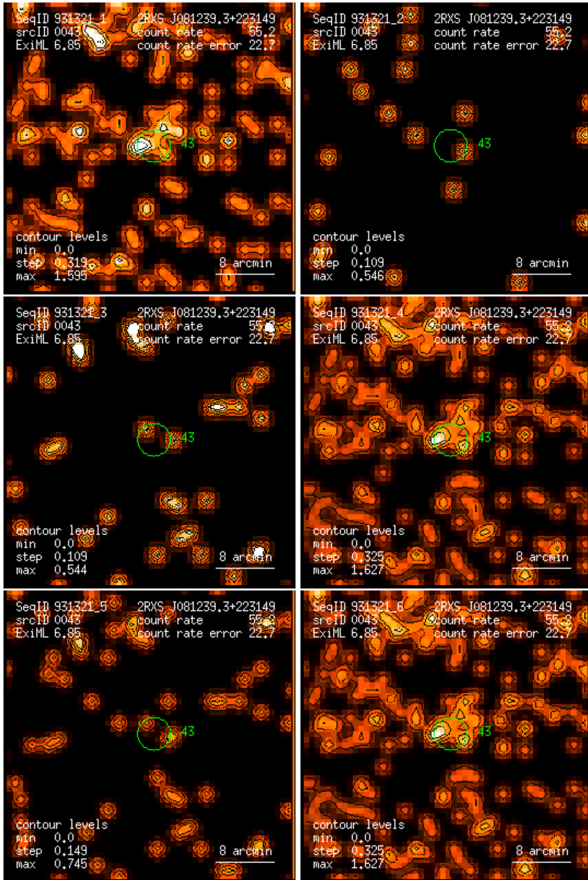
Figure 43: RASS 931321: detection 0043: band rate images, Gaussian filter: (1) PSPC channels 11 – 41, (2) 52 – 90, (3) 91 – 201, (4) 11 – 235, (5) 52 – 201, (6) 11 – 201. Broad band rates in counts/ks. Band rate contour levels in counts/ks/arcmin 2 .
