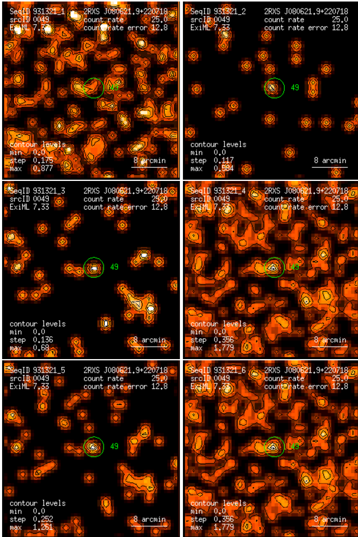
Figure 49: RASS 931321: detection 0049: band rate images, Gaussian filter: (1) PSPC channels 11 – 41, (2) 52 – 90, (3) 91 – 201, (4) 11 – 235, (5) 52 – 201, (6) 11 – 201. Broad band rates in counts/ks. Band rate contour levels in counts/ks/arcmin 2 .
