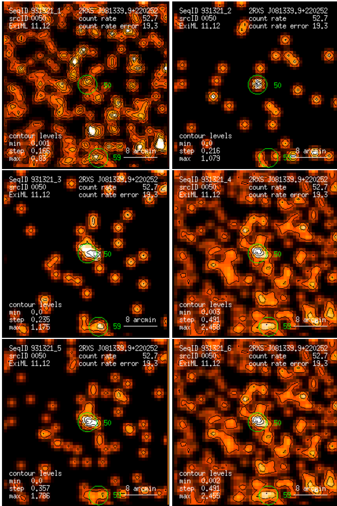
Figure 50: RASS 931321: detection 0050: band rate images, Gaussian filter: (1) PSPC channels 11 – 41, (2) 52 – 90, (3) 91 – 201, (4) 11 – 235, (5) 52 – 201, (6) 11 – 201. Broad band rates in counts/ks. Band rate contour levels in counts/ks/arcmin 2 .
