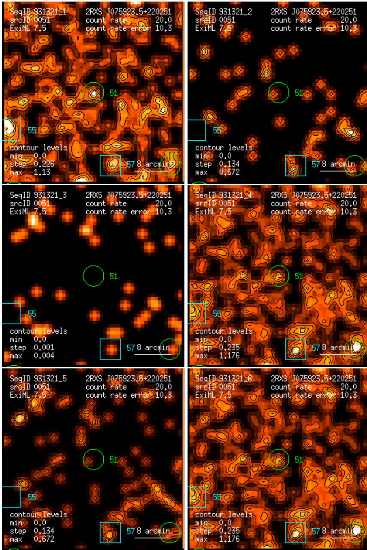
Figure 51: RASS 931321: detection 0051: band rate images, Gaussian filter: (1) PSPC channels 11 – 41, (2) 52 – 90, (3) 91 – 201, (4) 11 – 235, (5) 52 – 201, (6) 11 – 201. Broad band rates in counts/ks. Band rate contour levels in counts/ks/arcmin 2 .
