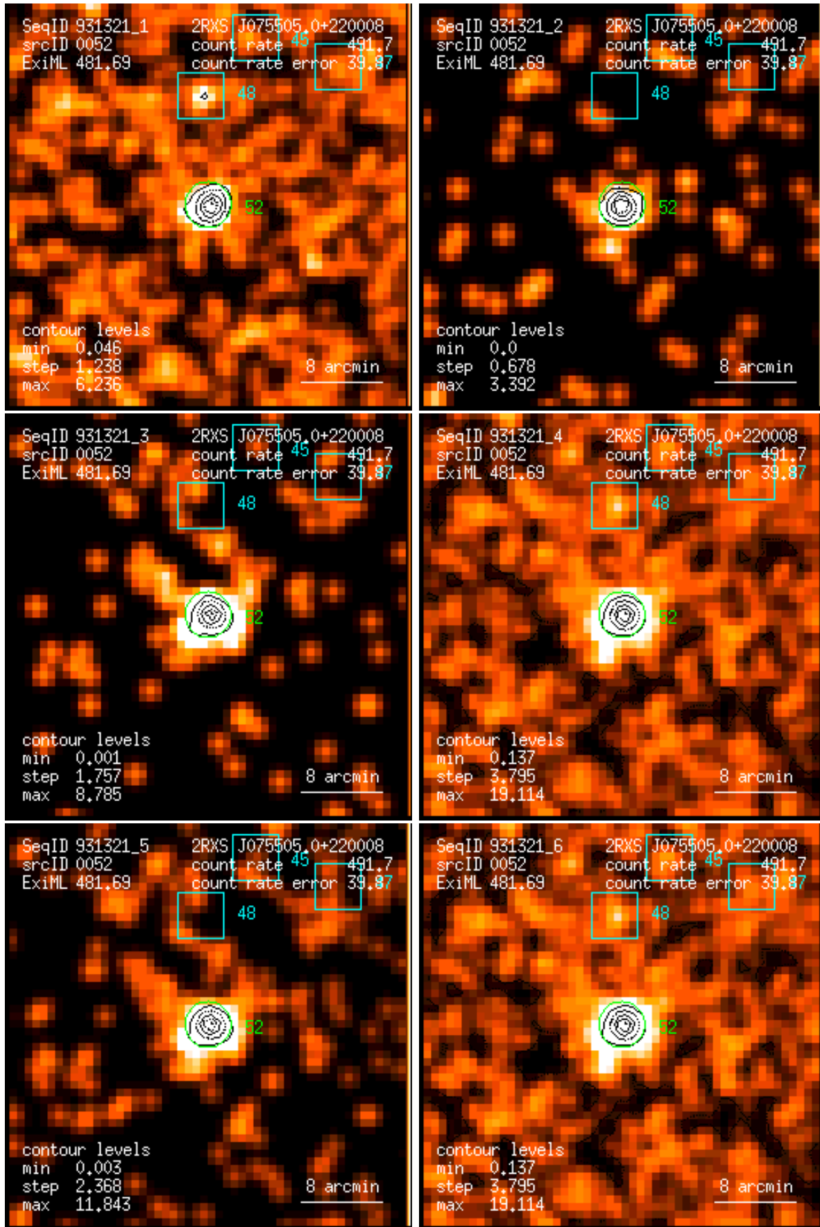
Figure 52: RASS 931321: detection 0052: band rate images, Gaussian filter: (1) PSPC channels 11 – 41, (2) 52 – 90, (3) 91 – 201, (4) 11 – 235, (5) 52 – 201, (6) 11 – 201. Broad band rates in counts/ks. Band rate contour levels in counts/ks/arcmin 2 .
