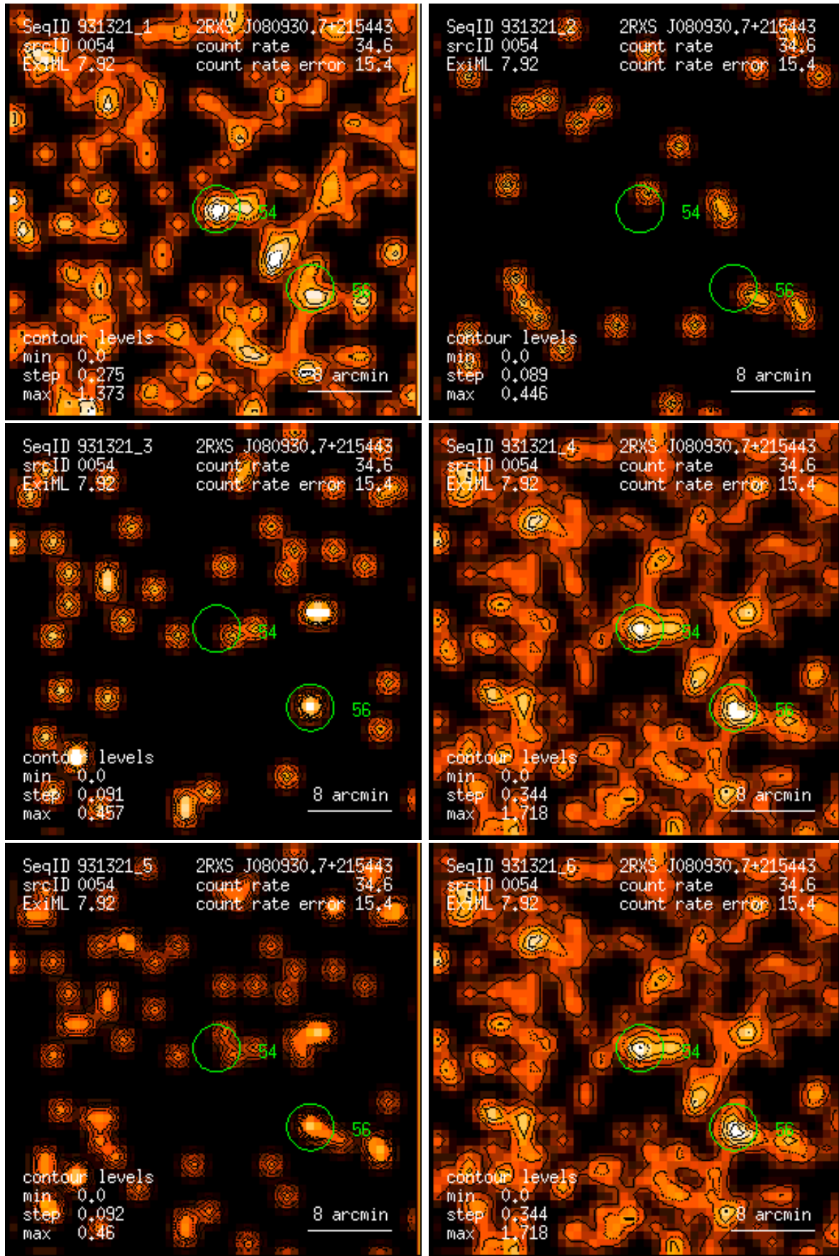
Figure 54: RASS 931321: detection 0054: band rate images, Gaussian filter: (1) PSPC channels 11 – 41, (2) 52 – 90, (3) 91 – 201, (4) 11 – 235, (5) 52 – 201, (6) 11 – 201. Broad band rates in counts/ks. Band rate contour levels in counts/ks/arcmin 2 .
