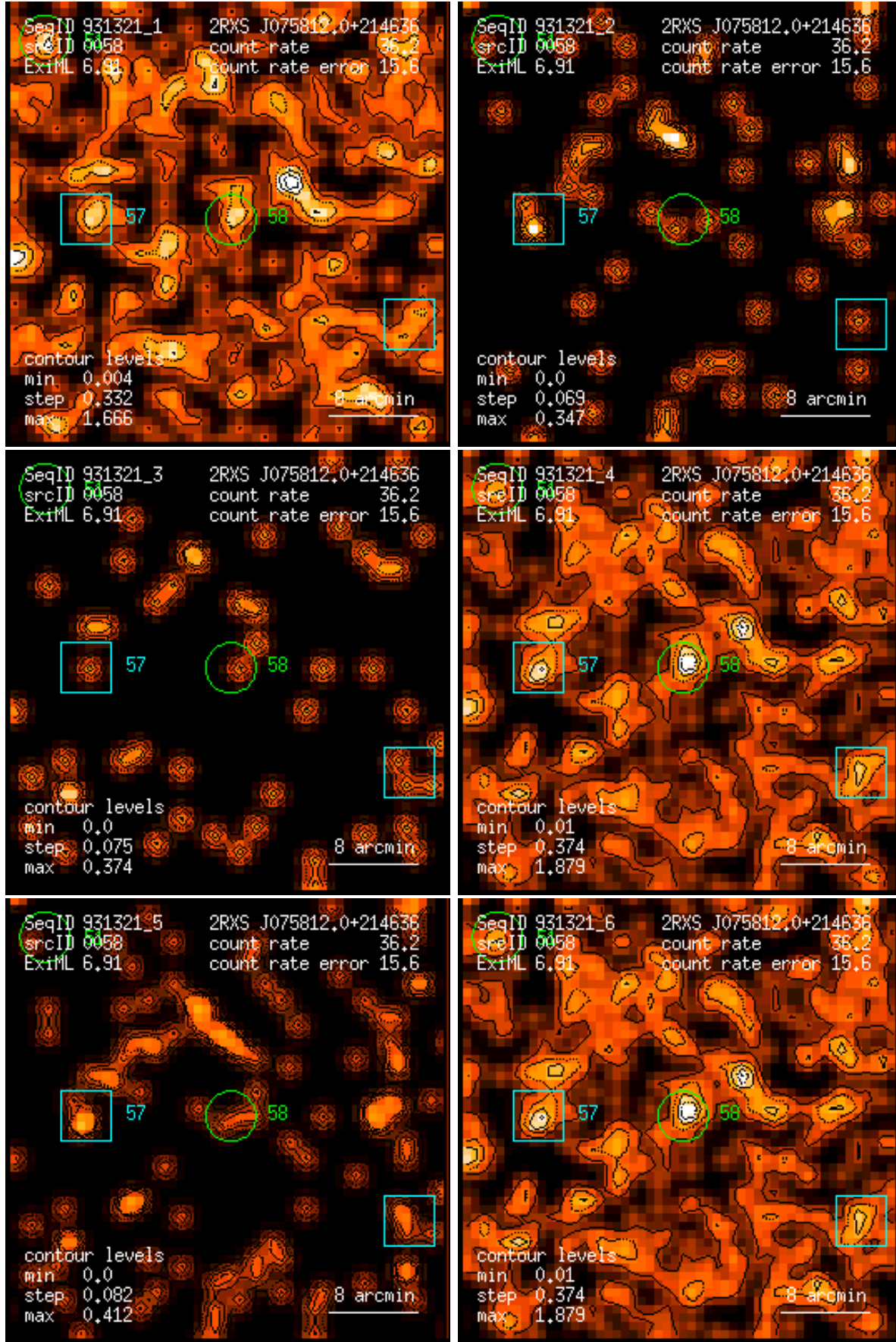
Figure 58: RASS 931321: detection 0058: band rate images, Gaussian filter: (1) PSPC channels 11 – 41, (2) 52 – 90, (3) 91 – 201, (4) 11 – 235, (5) 52 – 201, (6) 11 – 201. Broad band rates in counts/ks. Band rate contour levels in counts/ks/arcmin 2 .
