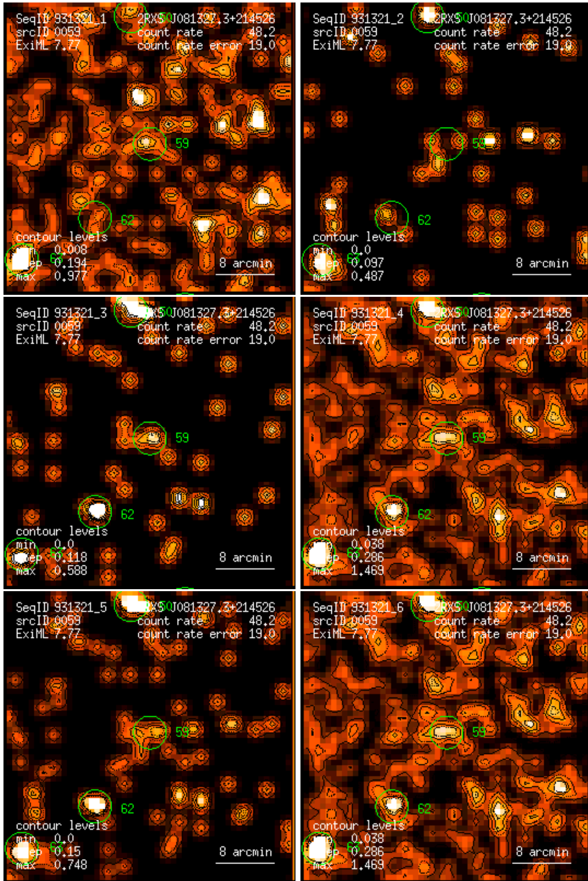
Figure 59: RASS 931321: detection 0059: band rate images, Gaussian filter: (1) PSPC channels 11 – 41, (2) 52 – 90, (3) 91 – 201, (4) 11 – 235, (5) 52 – 201, (6) 11 – 201. Broad band rates in counts/ks. Band rate contour levels in counts/ks/arcmin 2 .
