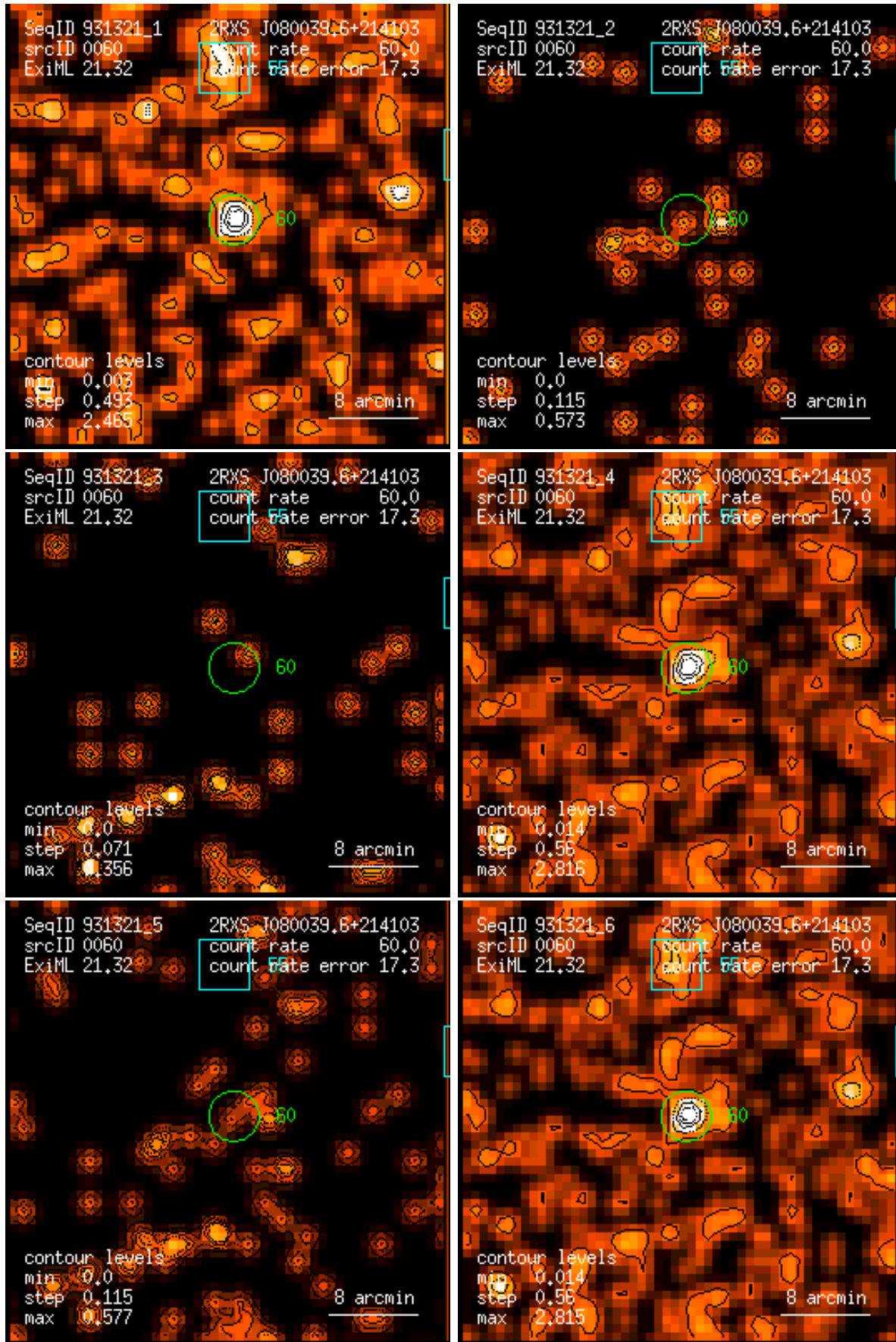
Figure 60: RASS 931321: detection 0060: band rate images, Gaussian filter: (1) PSPC channels 11 – 41, (2) 52 – 90, (3) 91 – 201, (4) 11 – 235, (5) 52 – 201, (6) 11 – 201. Broad band rates in counts/ks. Band rate contour levels in counts/ks/arcmin 2 .
