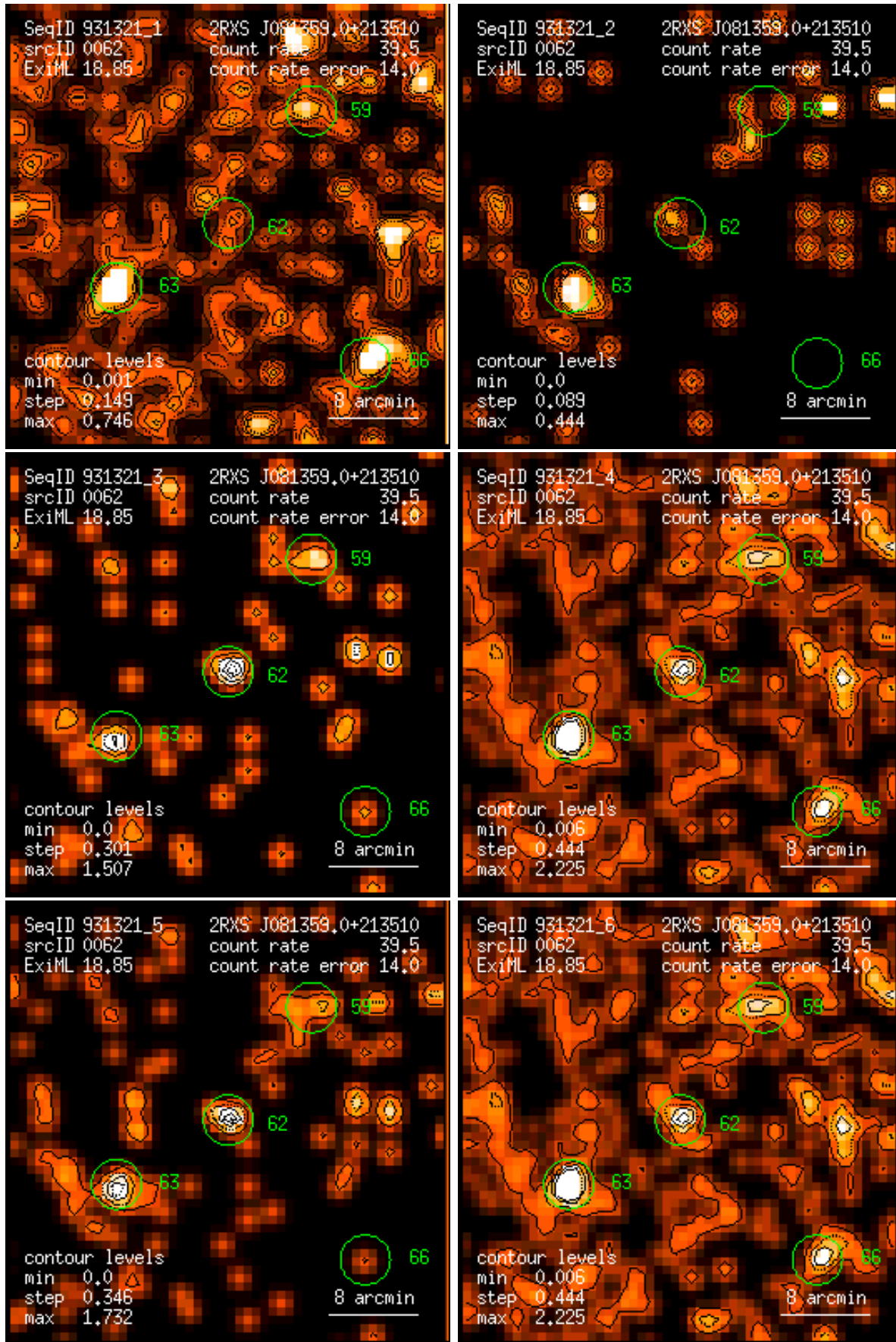
Figure 62: RASS 931321: detection 0062: band rate images, Gaussian filter: (1) PSPC channels 11 – 41, (2) 52 – 90, (3) 91 – 201, (4) 11 – 235, (5) 52 – 201, (6) 11 – 201. Broad band rates in counts/ks. Band rate contour levels in counts/ks/arcmin 2 .
