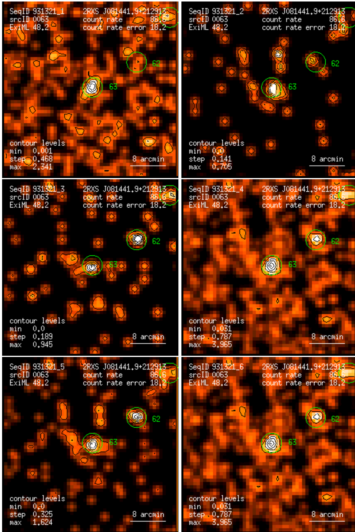
Figure 63: RASS 931321: detection 0063: band rate images, Gaussian filter: (1) PSPC channels 11 – 41, (2) 52 – 90, (3) 91 – 201, (4) 11 – 235, (5) 52 – 201, (6) 11 – 201. Broad band rates in counts/ks. Band rate contour levels in counts/ks/arcmin 2 .
