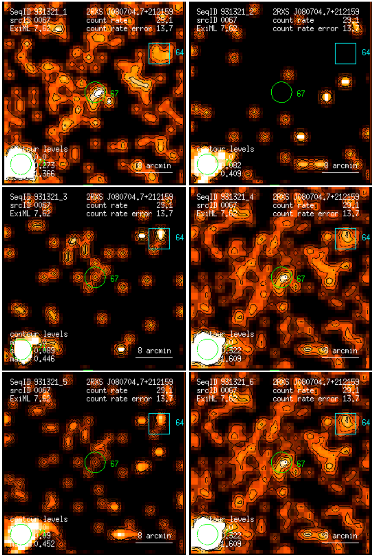
Figure 67: RASS 931321: detection 0067: band rate images, Gaussian filter: (1) PSPC channels 11 – 41, (2) 52 – 90, (3) 91 – 201, (4) 11 – 235, (5) 52 – 201, (6) 11 – 201. Broad band rates in counts/ks. Band rate contour levels in counts/ks/arcmin 2 .
