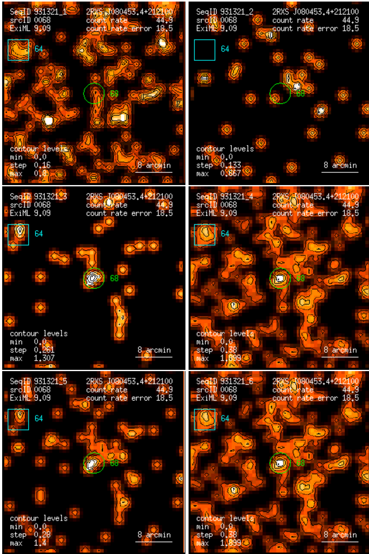
Figure 68: RASS 931321: detection 0068: band rate images, Gaussian filter: (1) PSPC channels 11 – 41, (2) 52 – 90, (3) 91 – 201, (4) 11 – 235, (5) 52 – 201, (6) 11 – 201. Broad band rates in counts/ks. Band rate contour levels in counts/ks/arcmin 2 .
