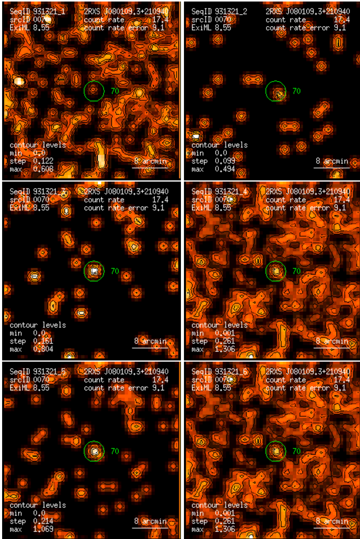
Figure 70: RASS 931321: detection 0070: band rate images, Gaussian filter: (1) PSPC channels 11 – 41, (2) 52 – 90, (3) 91 – 201, (4) 11 – 235, (5) 52 – 201, (6) 11 – 201. Broad band rates in counts/ks. Band rate contour levels in counts/ks/arcmin 2 .
