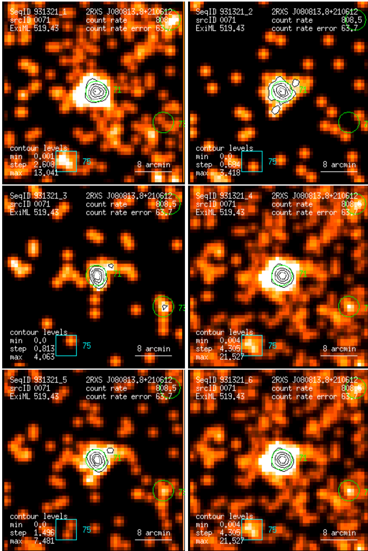
Figure 71: RASS 931321: detection 0071: band rate images, Gaussian filter: (1) PSPC channels 11 – 41, (2) 52 – 90, (3) 91 – 201, (4) 11 – 235, (5) 52 – 201, (6) 11 – 201. Broad band rates in counts/ks. Band rate contour levels in counts/ks/arcmin 2 .
