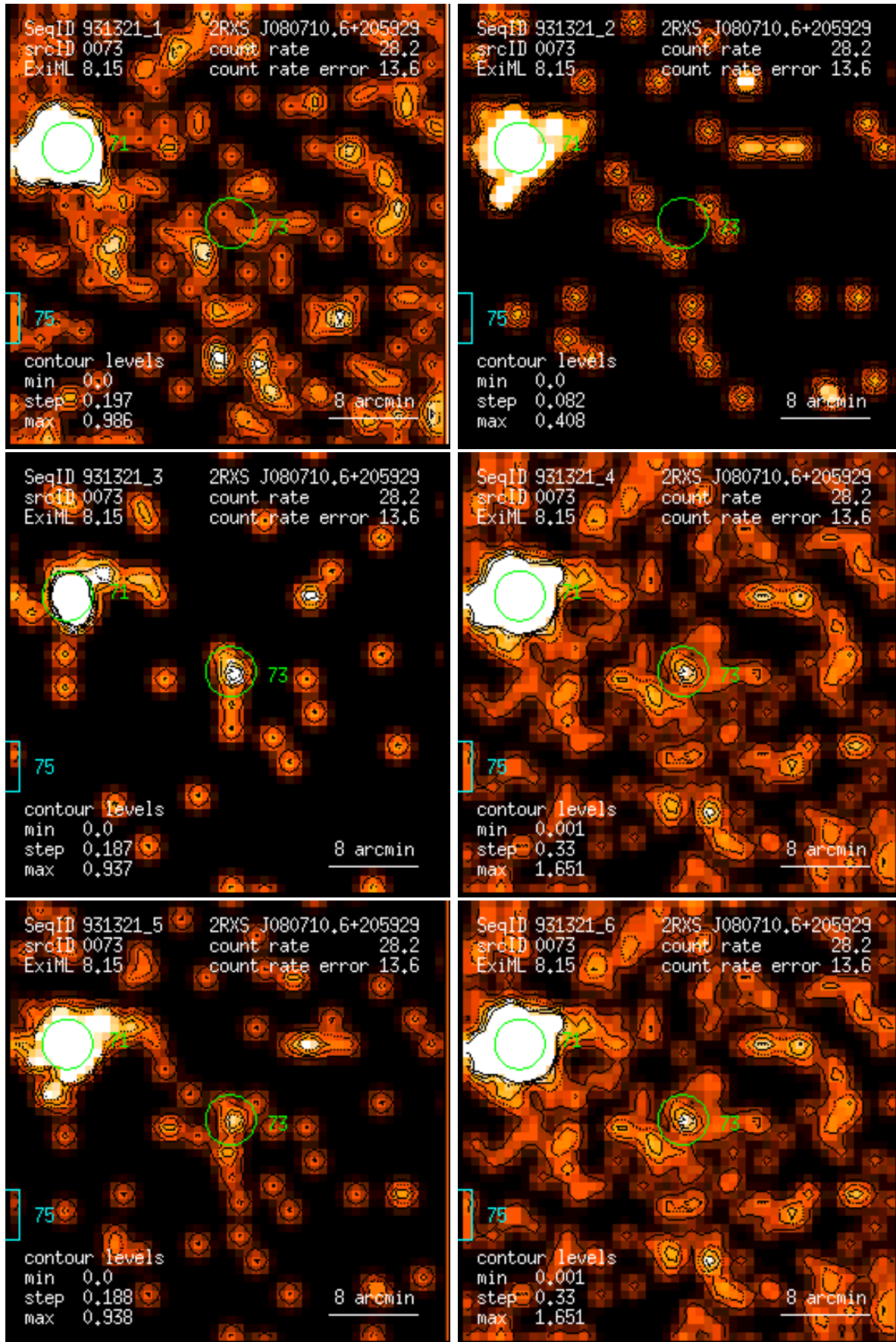
Figure 73: RASS 931321: detection 0073: band rate images, Gaussian filter: (1) PSPC channels 11 – 41, (2) 52 – 90, (3) 91 – 201, (4) 11 – 235, (5) 52 – 201, (6) 11 – 201. Broad band rates in counts/ks. Band rate contour levels in counts/ks/arcmin 2 .
