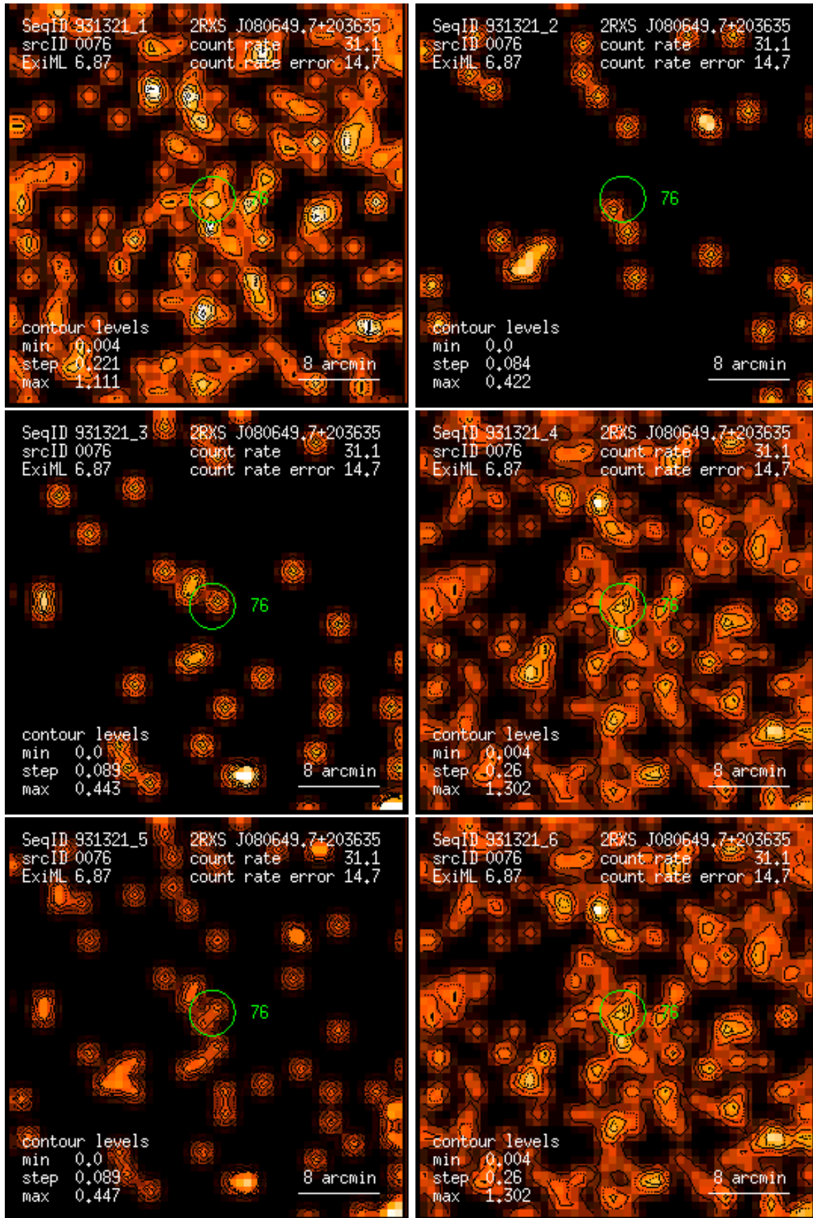
Figure 76: RASS 931321: detection 0076: band rate images, Gaussian filter: (1) PSPC channels 11 – 41, (2) 52 – 90, (3) 91 – 201, (4) 11 – 235, (5) 52 – 201, (6) 11 – 201. Broad band rates in counts/ks. Band rate contour levels in counts/ks/arcmin 2 .
