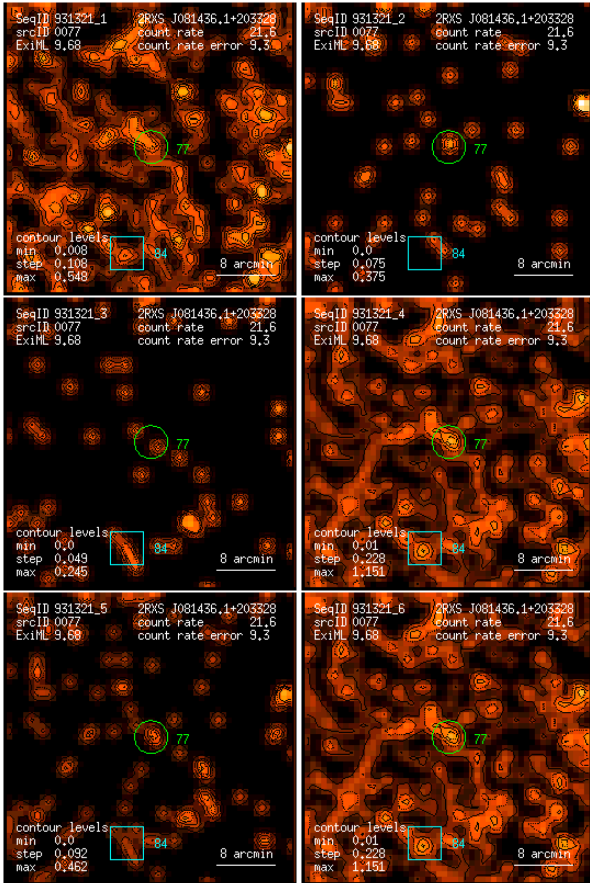
Figure 77: RASS 931321: detection 0077: band rate images, Gaussian filter: (1) PSPC channels 11 – 41, (2) 52 – 90, (3) 91 – 201, (4) 11 – 235, (5) 52 – 201, (6) 11 – 201. Broad band rates in counts/ks. Band rate contour levels in counts/ks/arcmin 2 .
