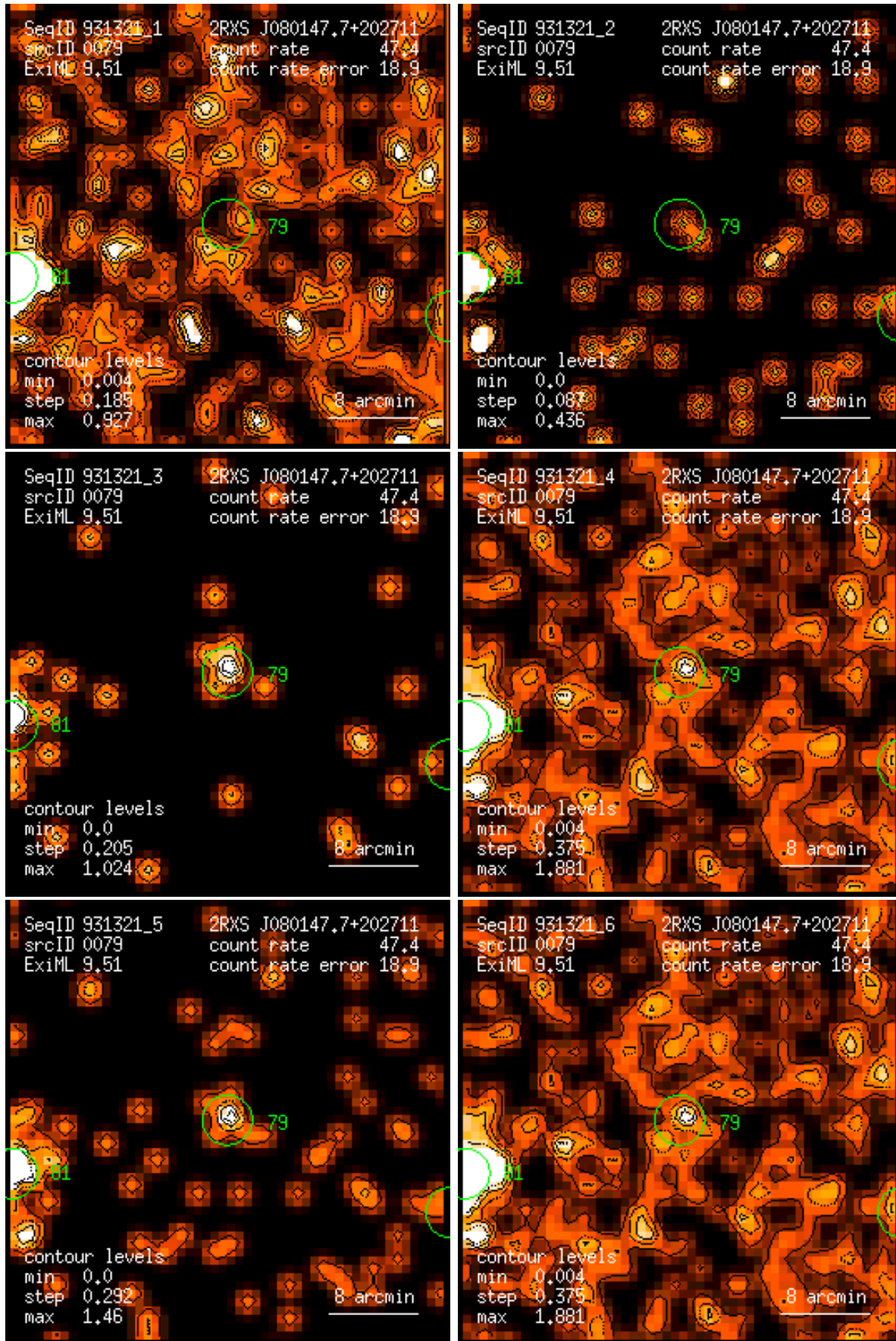
Figure 79: RASS 931321: detection 0079: band rate images, Gaussian filter: (1) PSPC channels 11 – 41, (2) 52 – 90, (3) 91 – 201, (4) 11 – 235, (5) 52 – 201, (6) 11 – 201. Broad band rates in counts/ks. Band rate contour levels in counts/ks/arcmin 2 .
