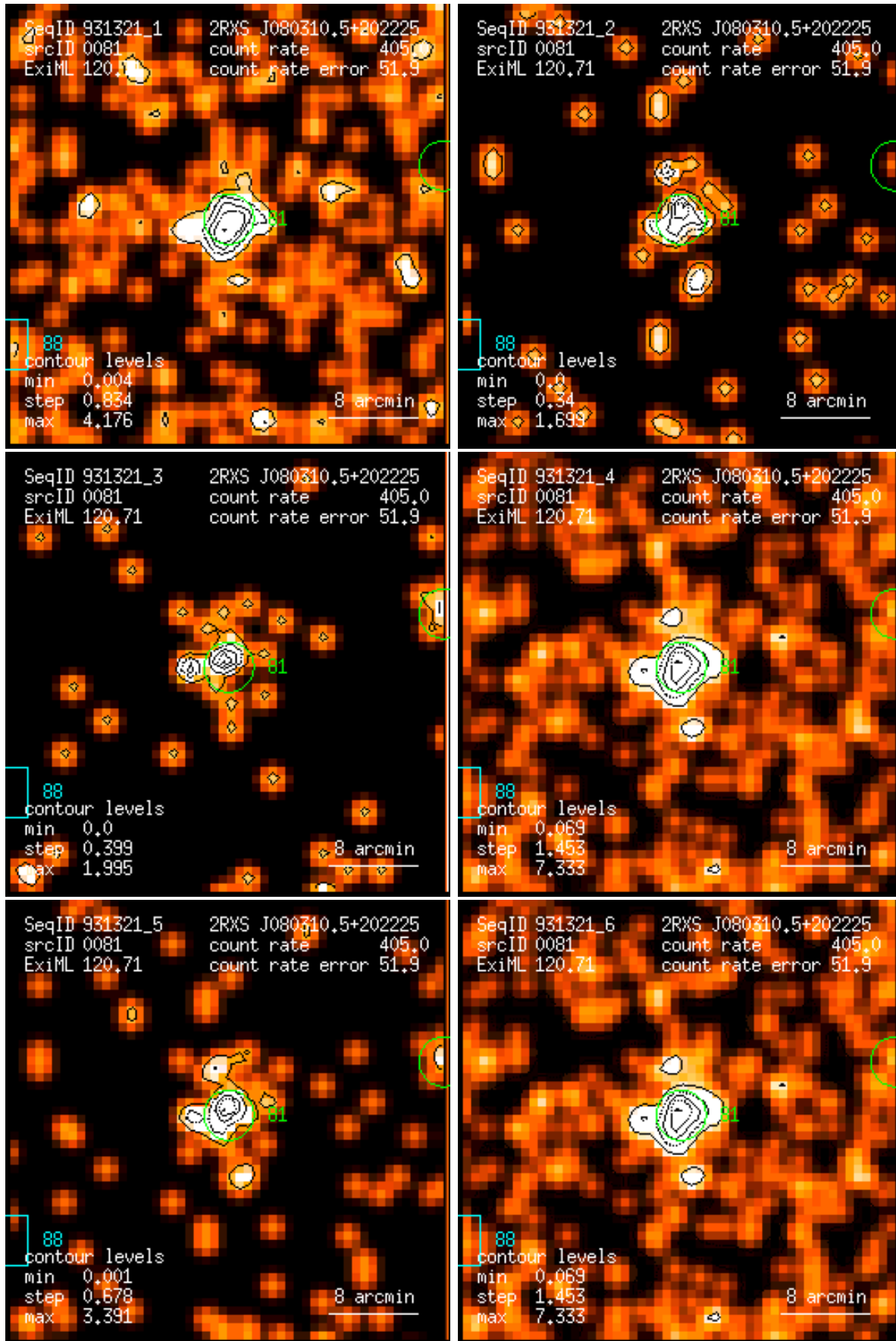
Figure 81: RASS 931321: detection 0081: band rate images, Gaussian filter: (1) PSPC channels 11 – 41, (2) 52 – 90, (3) 91 – 201, (4) 11 – 235, (5) 52 – 201, (6) 11 – 201. Broad band rates in counts/ks. Band rate contour levels in counts/ks/arcmin 2 .
