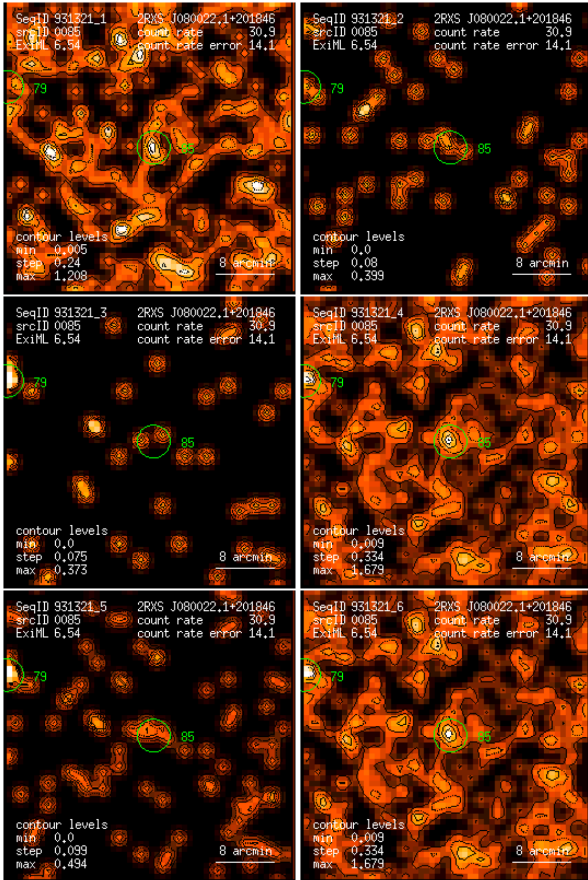
Figure 85: RASS 931321: detection 0085: band rate images, Gaussian filter: (1) PSPC channels 11 – 41, (2) 52 – 90, (3) 91 – 201, (4) 11 – 235, (5) 52 – 201, (6) 11 – 201. Broad band rates in counts/ks. Band rate contour levels in counts/ks/arcmin 2 .
