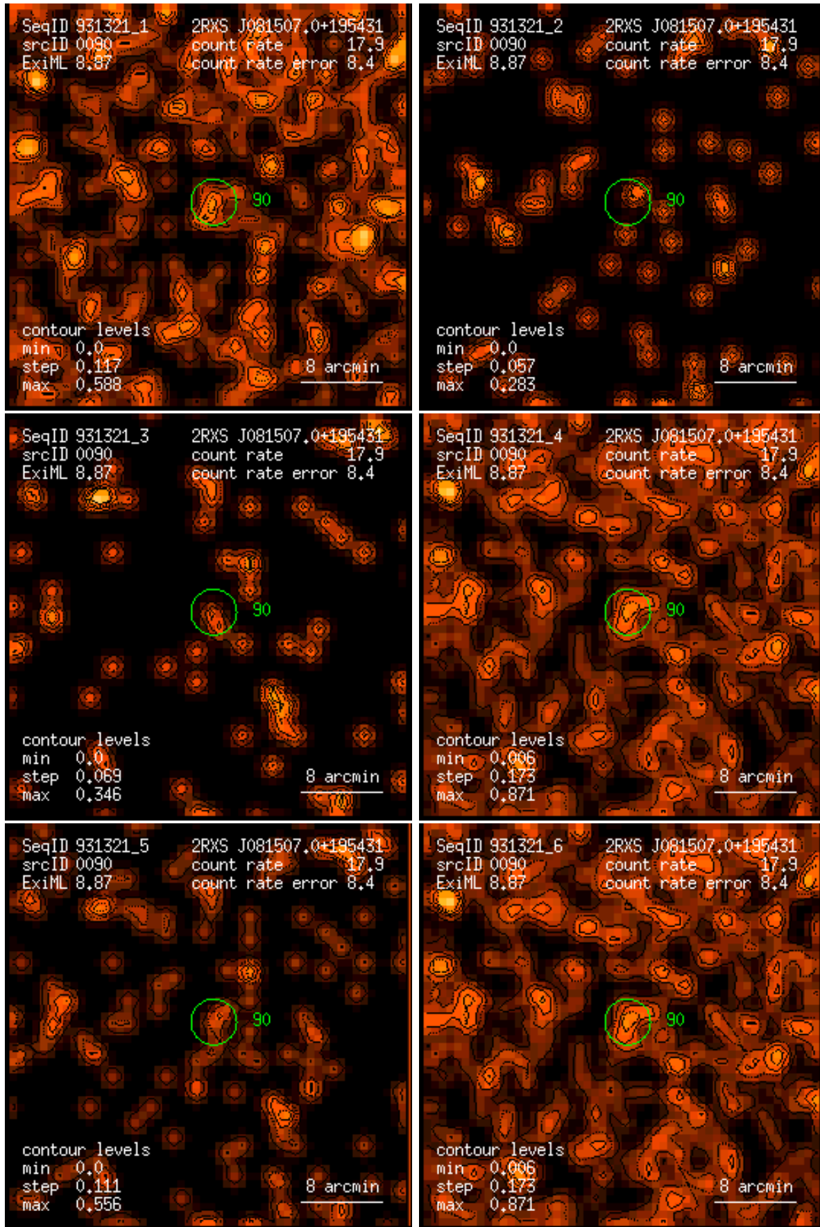
Figure 90: RASS 931321: detection 0090: band rate images, Gaussian filter: (1) PSPC channels 11 – 41, (2) 52 – 90, (3) 91 – 201, (4) 11 – 235, (5) 52 – 201, (6) 11 – 201. Broad band rates in counts/ks. Band rate contour levels in counts/ks/arcmin 2 .
