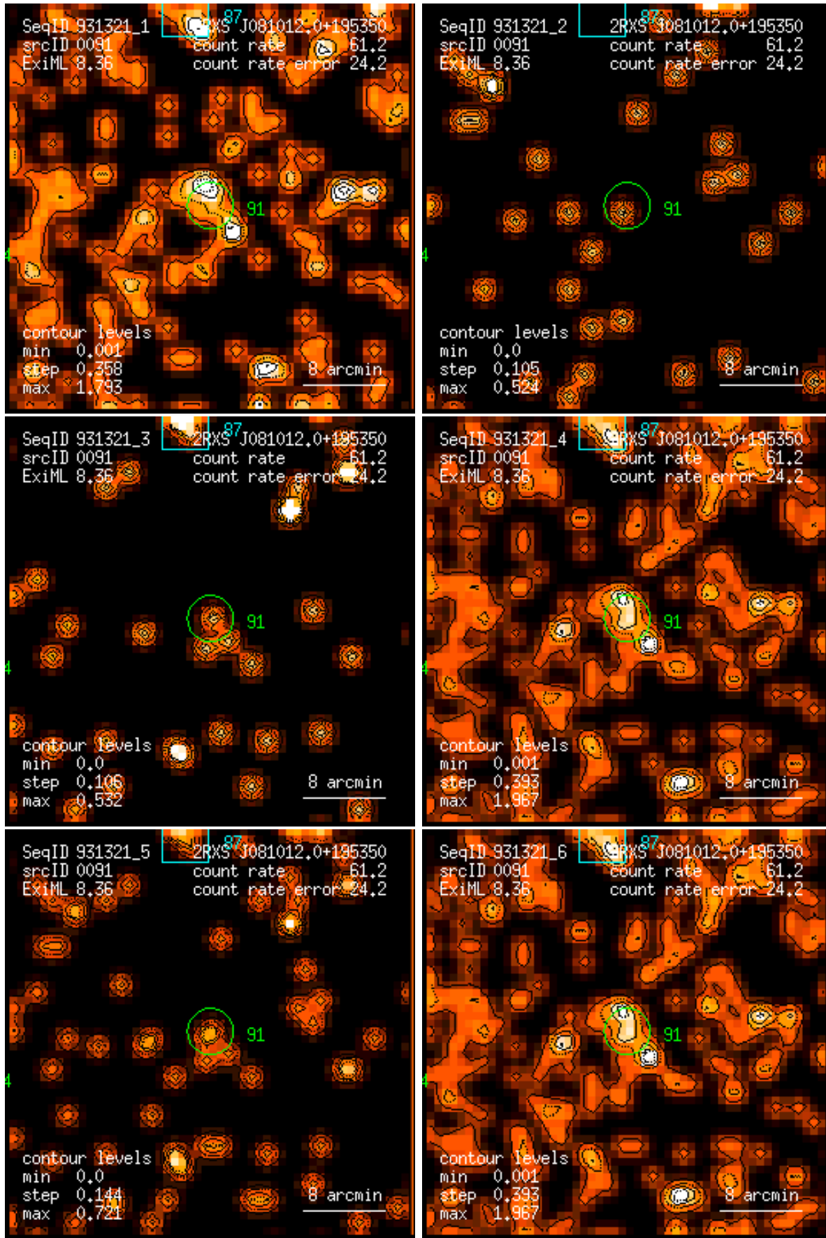
Figure 91: RASS 931321: detection 0091: band rate images, Gaussian filter: (1) PSPC channels 11 – 41, (2) 52 – 90, (3) 91 – 201, (4) 11 – 235, (5) 52 – 201, (6) 11 – 201. Broad band rates in counts/ks. Band rate contour levels in counts/ks/arcmin 2 .
