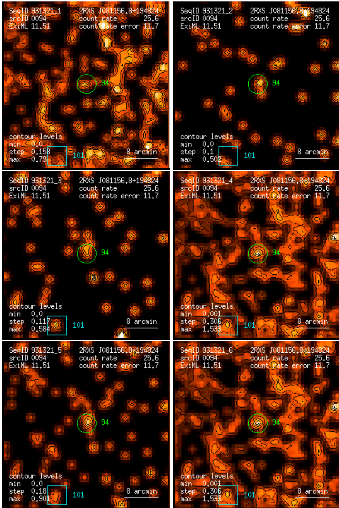
Figure 94: RASS 931321: detection 0094: band rate images, Gaussian filter: (1) PSPC channels 11 – 41, (2) 52 – 90, (3) 91 – 201, (4) 11 – 235, (5) 52 – 201, (6) 11 – 201. Broad band rates in counts/ks. Band rate contour levels in counts/ks/arcmin 2 .
