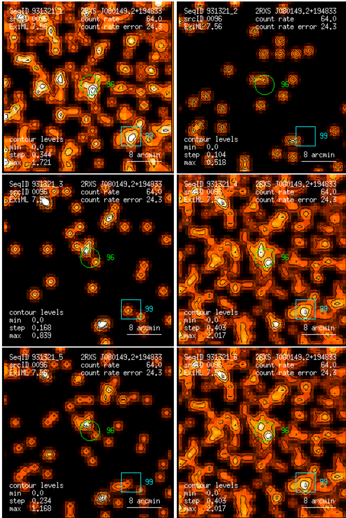
Figure 96: RASS 931321: detection 0096: band rate images, Gaussian filter: (1) PSPC channels 11 – 41, (2) 52 – 90, (3) 91 – 201, (4) 11 – 235, (5) 52 – 201, (6) 11 – 201. Broad band rates in counts/ks. Band rate contour levels in counts/ks/arcmin 2 .
