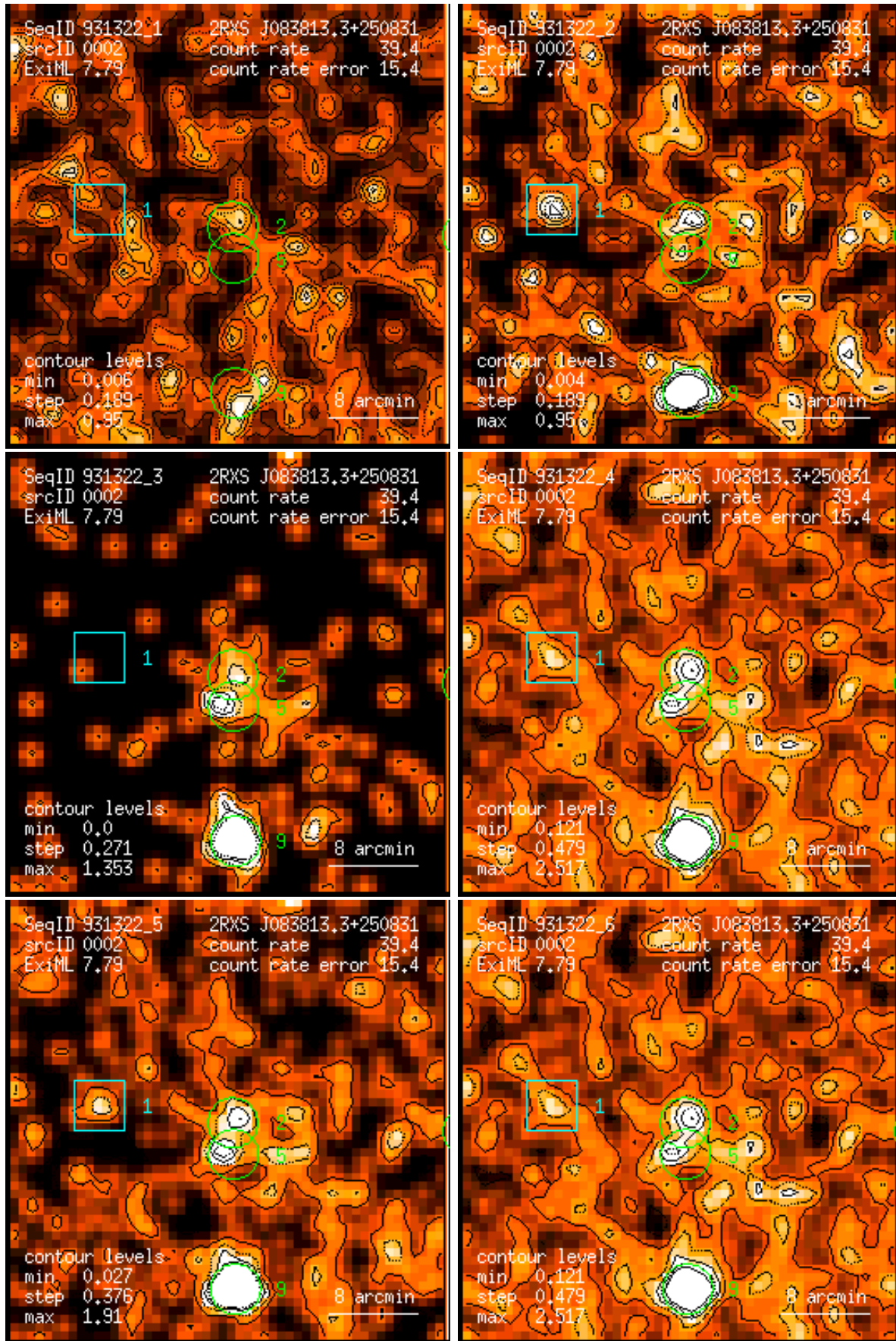
Figure 2: RASS 931322: detection 0002: band rate images, Gaussian filter: (1) PSPC channels 11 – 41, (2) 52 – 90, (3) 91 – 201, (4) 11 – 235, (5) 52 – 201, (6) 11 – 201. Broad band rates in counts/ks. Band rate contour levels in counts/ks/arcmin 2 .
