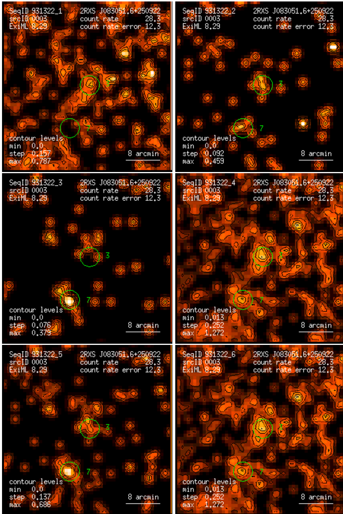
Figure 3: RASS 931322: detection 0003: band rate images, Gaussian filter: (1) PSPC channels 11 – 41, (2) 52 – 90, (3) 91 – 201, (4) 11 – 235, (5) 52 – 201, (6) 11 – 201. Broad band rates in counts/ks. Band rate contour levels in counts/ks/arcmin 2 .
