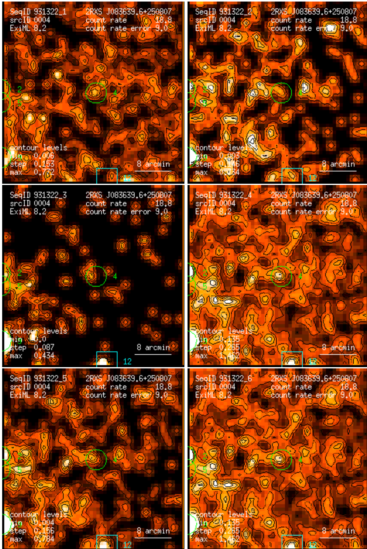
Figure 4: RASS 931322: detection 0004: band rate images, Gaussian filter: (1) PSPC channels 11 – 41, (2) 52 – 90, (3) 91 – 201, (4) 11 – 235, (5) 52 – 201, (6) 11 – 201. Broad band rates in counts/ks. Band rate contour levels in counts/ks/arcmin 2 .
