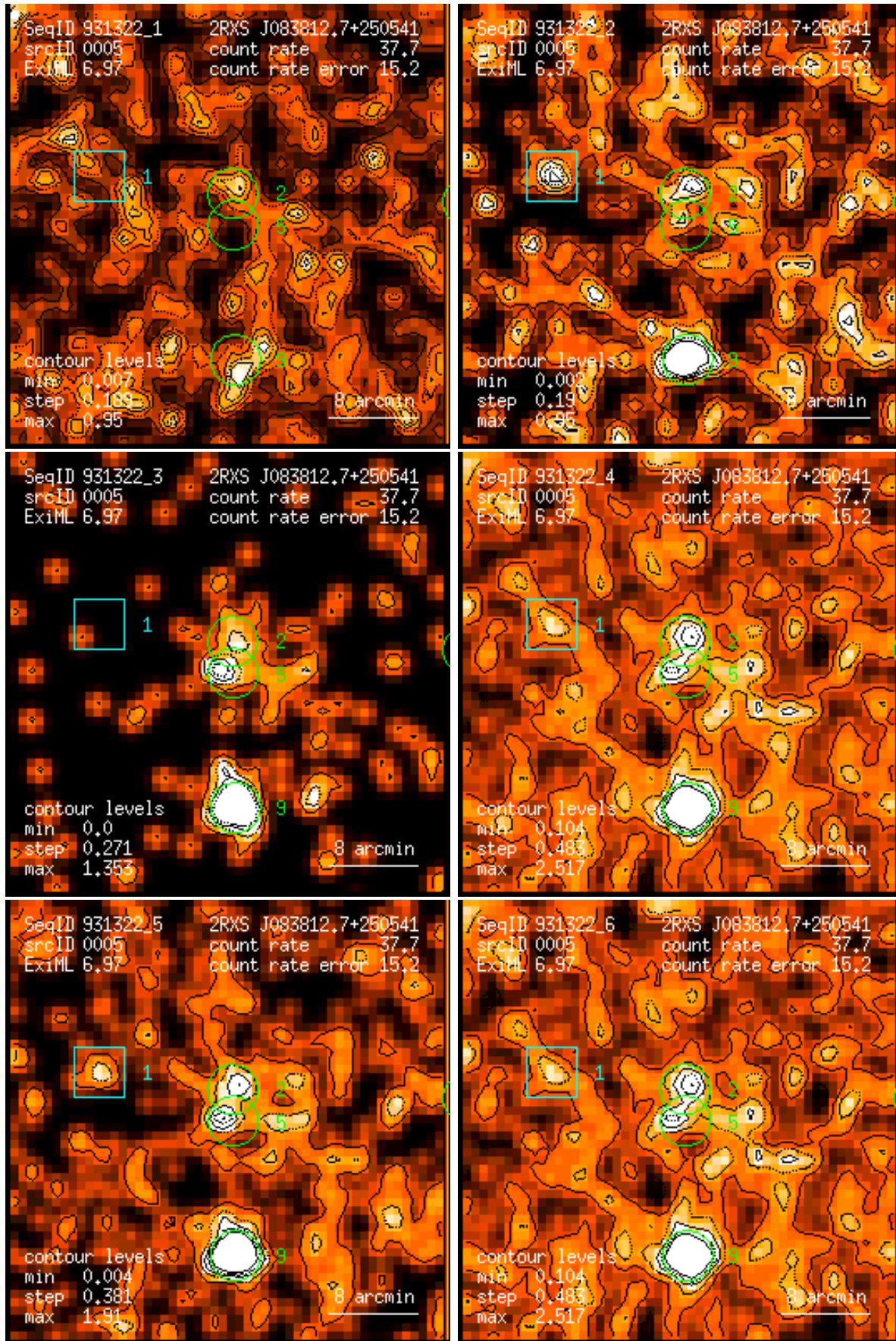
Figure 5: RASS 931322: detection 0005: band rate images, Gaussian filter: (1) PSPC channels 11 – 41, (2) 52 – 90, (3) 91 – 201, (4) 11 – 235, (5) 52 – 201, (6) 11 – 201. Broad band rates in counts/ks. Band rate contour levels in counts/ks/arcmin 2 .
