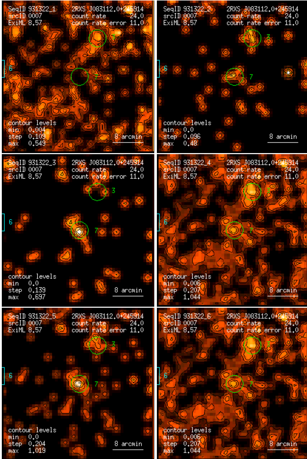
Figure 7: RASS 931322: detection 0007: band rate images, Gaussian filter: (1) PSPC channels 11 – 41, (2) 52 – 90, (3) 91 – 201, (4) 11 – 235, (5) 52 – 201, (6) 11 – 201. Broad band rates in counts/ks. Band rate contour levels in counts/ks/arcmin 2 .
